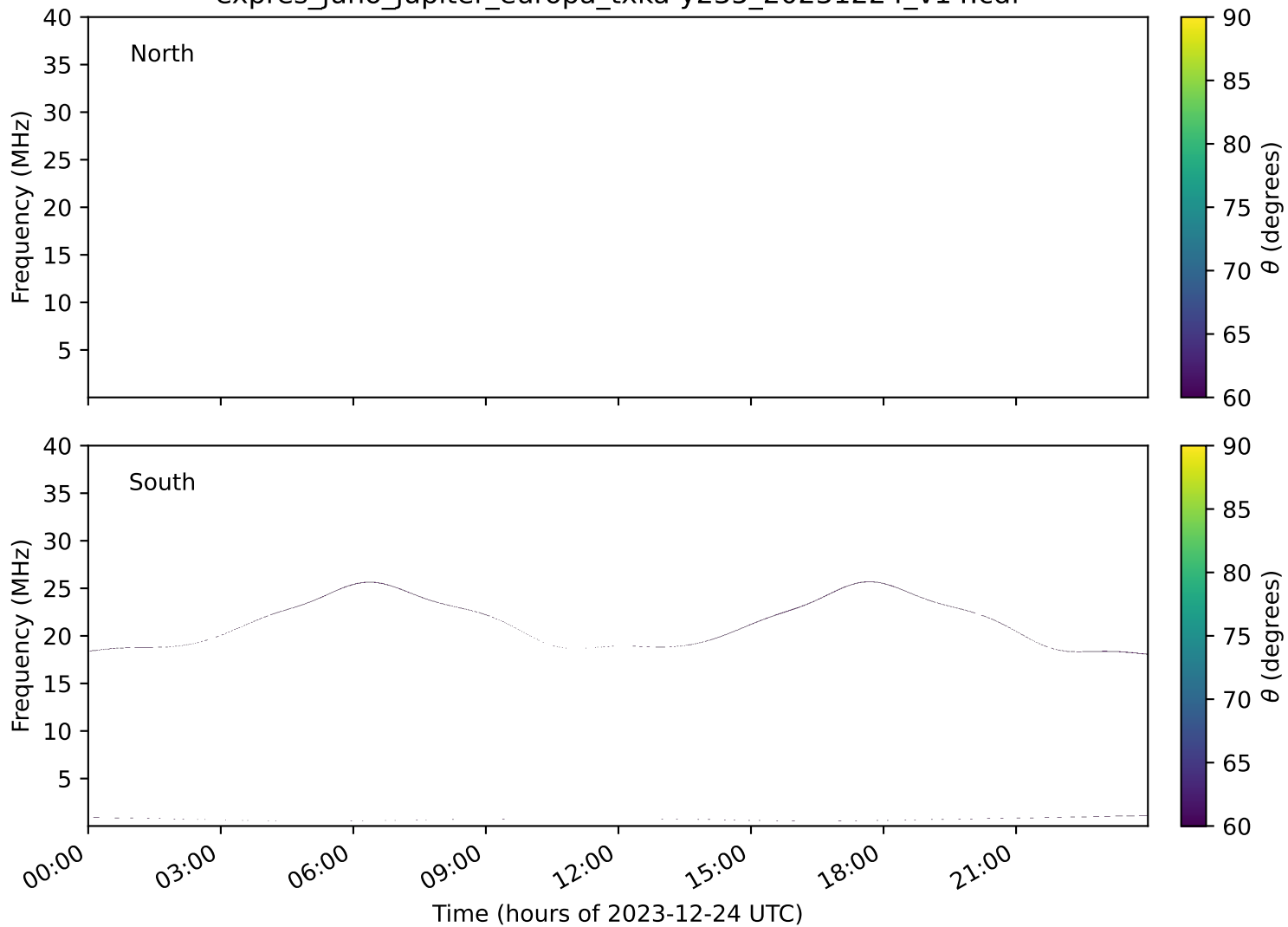
expres_juno_jupiter_europa_txka-y235_20231224_v14.cdf
