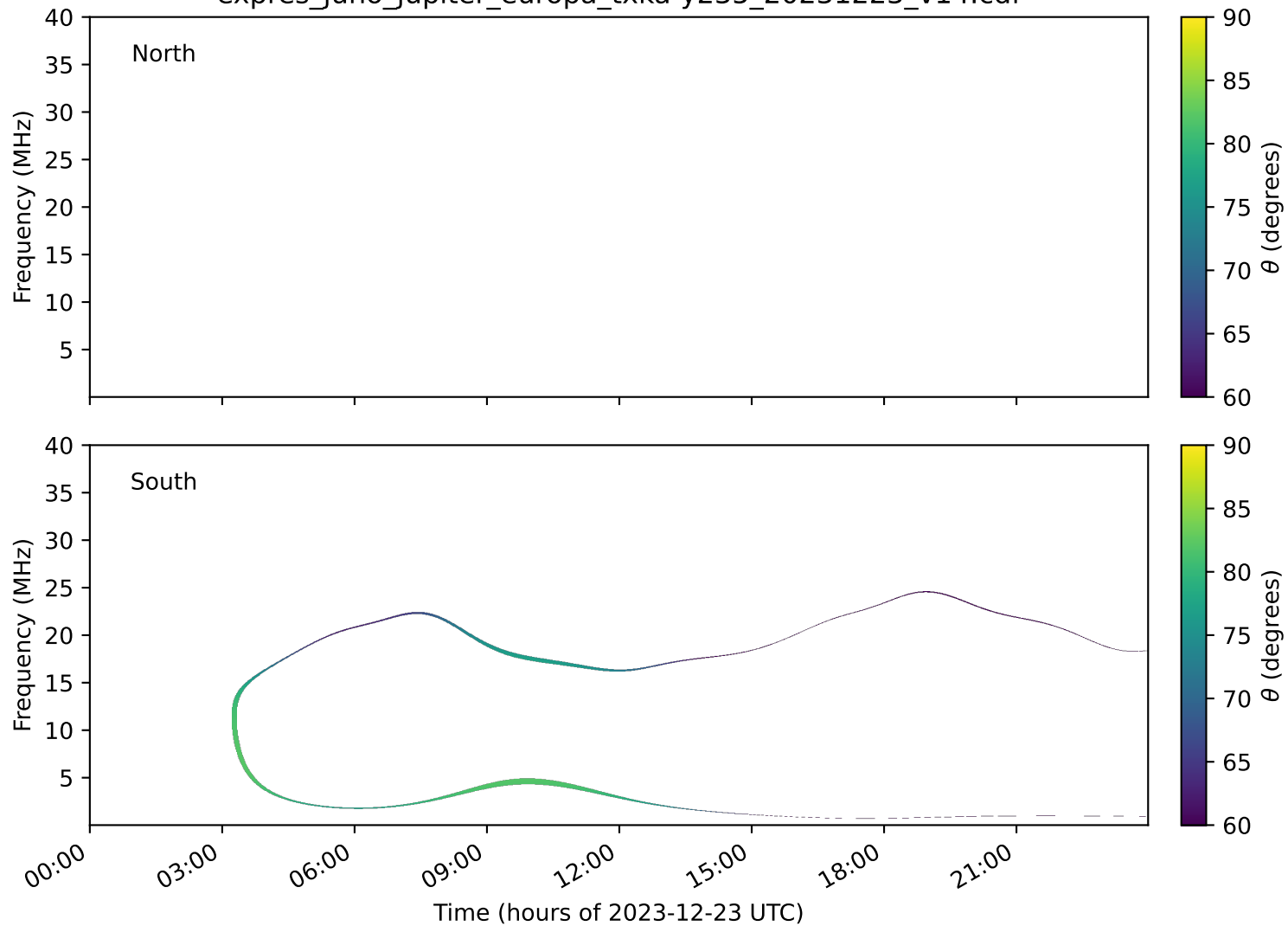
expres_juno_jupiter_europa_txka-y235_20231223_v14.cdf
