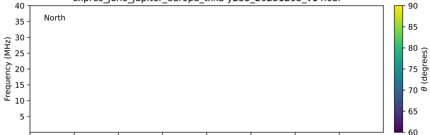
expres_juno_jupiter_europa_txka-y235_20231203_v14.cdf
