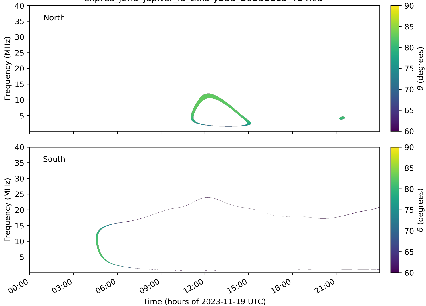
expres_juno_jupiter_io_txka-y235_20231119_v14.cdf
