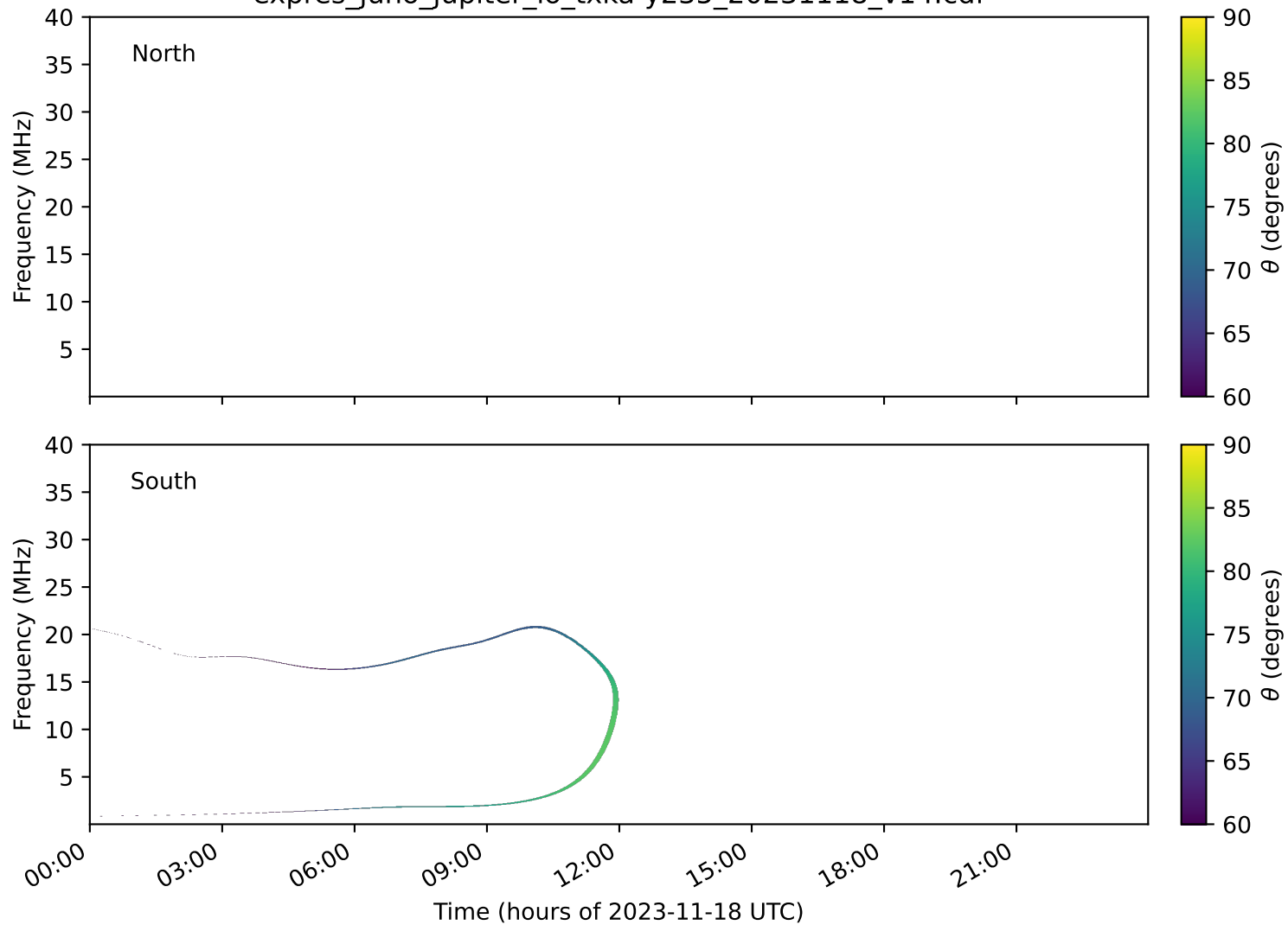
expres_juno_jupiter_io_txka-y235_20231118_v14.cdf
