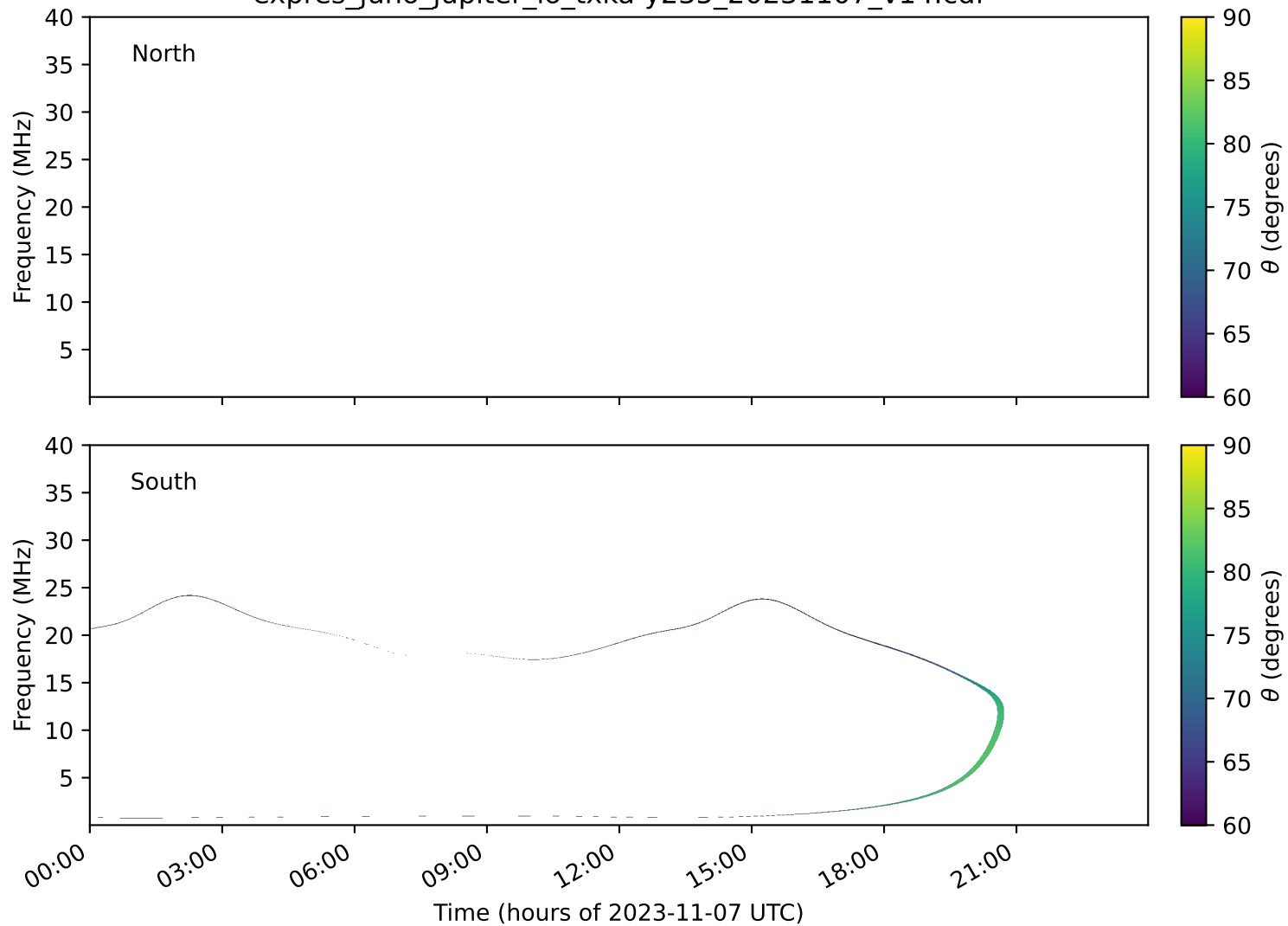
expres_juno_jupiter_io_txka-y235_20231107_v14.cdf
