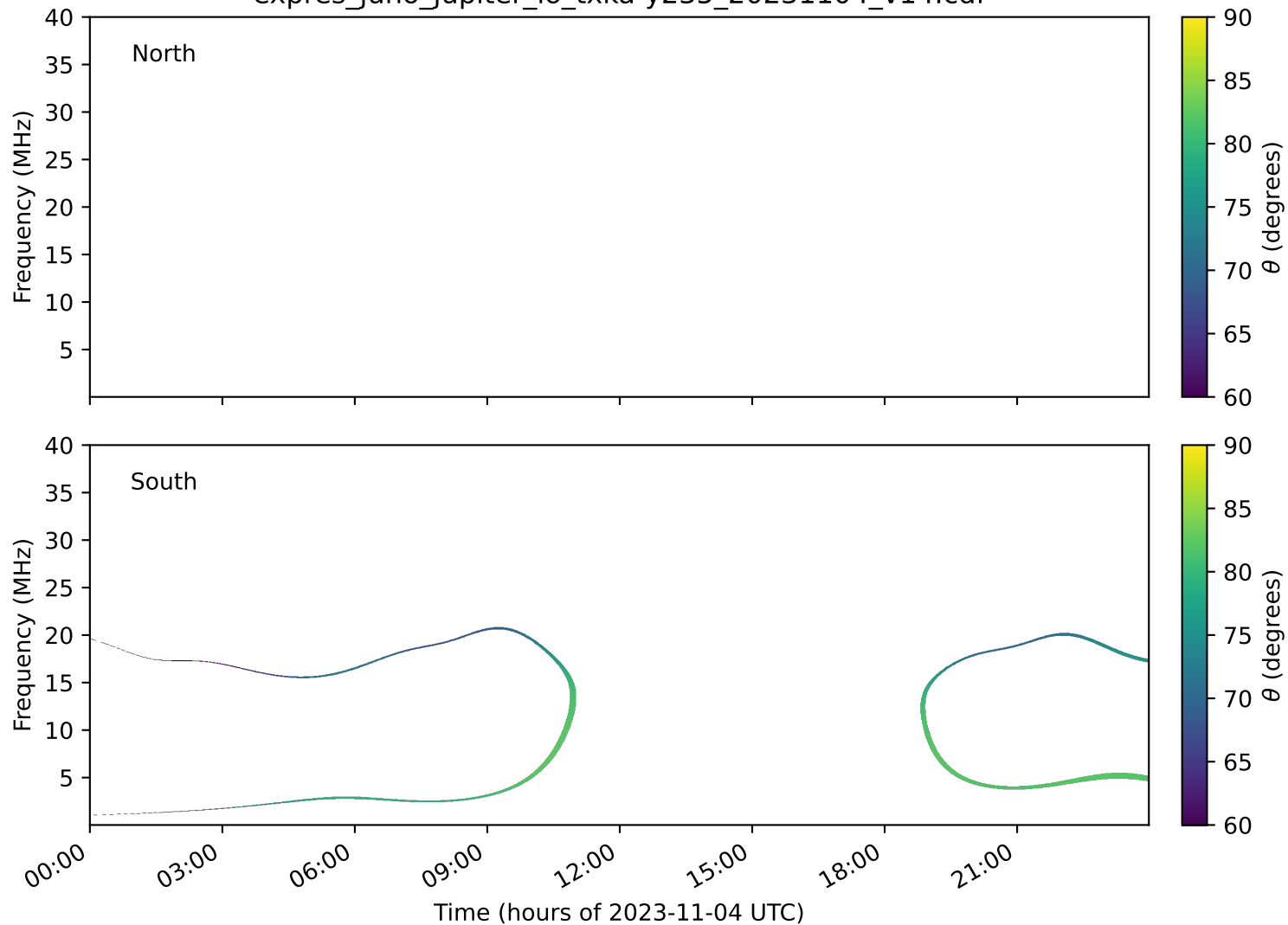
expres_juno_jupiter_io_txka-y235_20231104_v14.cdf
