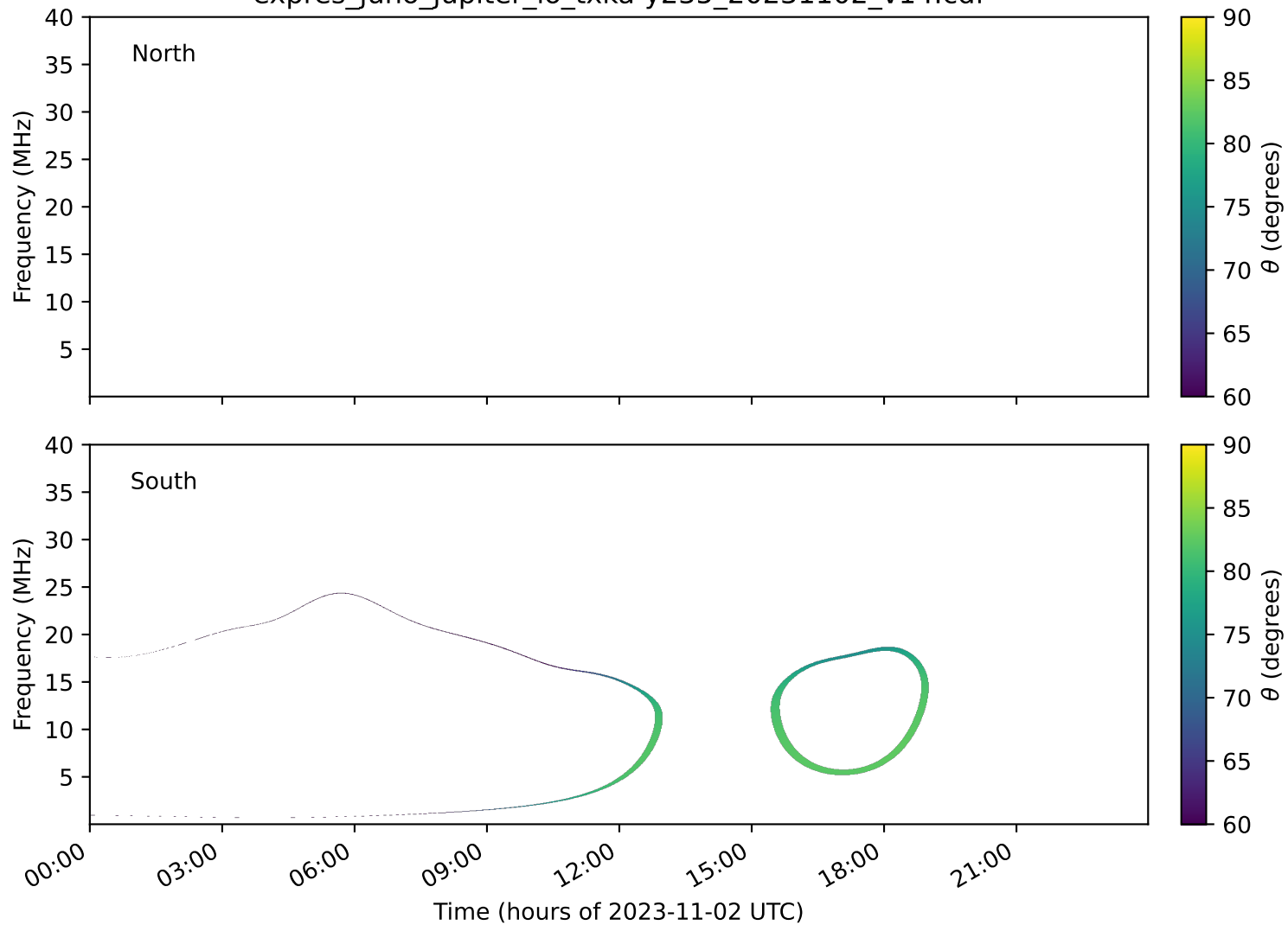
expres_juno_jupiter_io_txka-y235_20231102_v14.cdf
