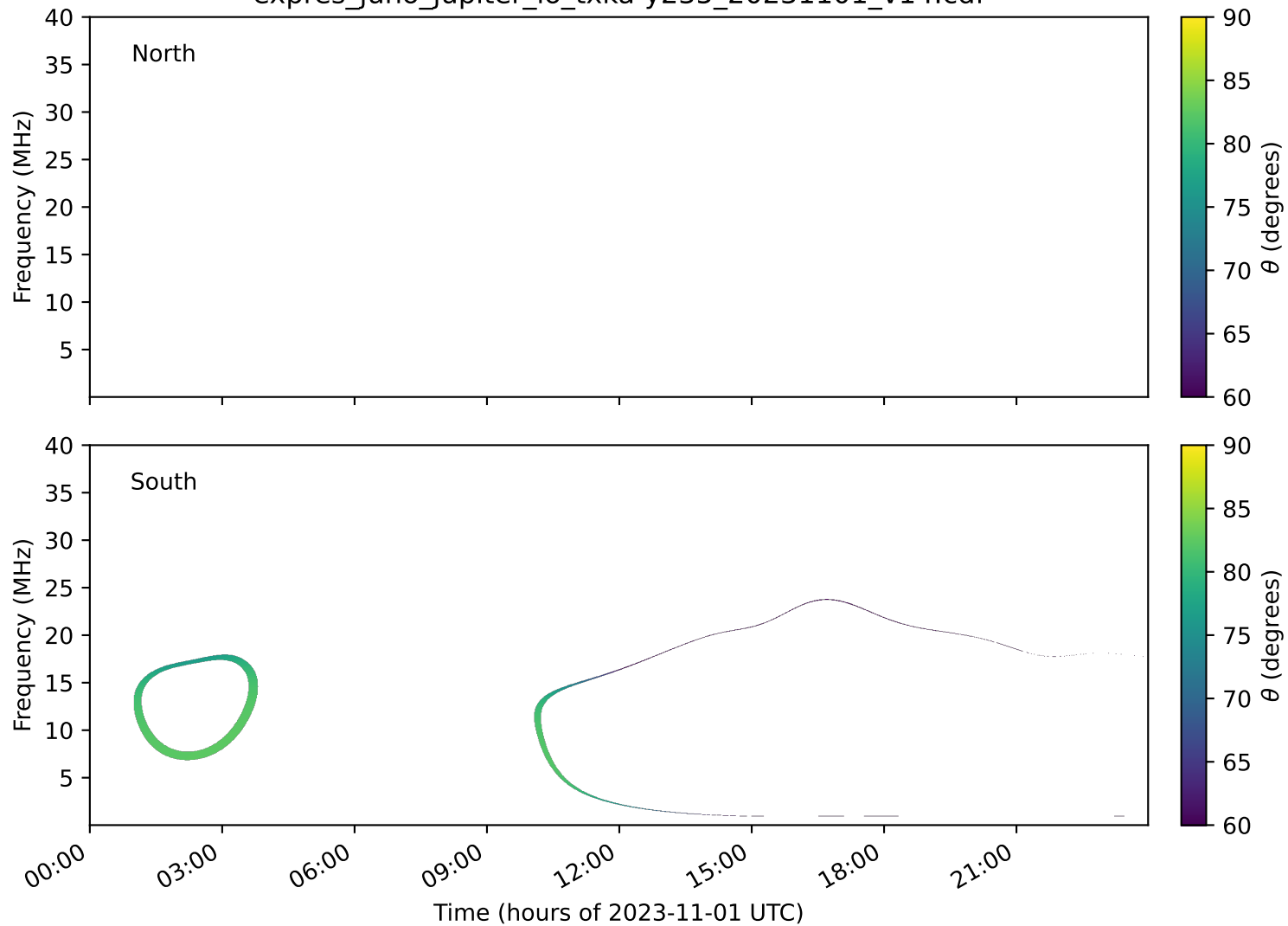
expres_juno_jupiter_io_txka-y235_20231101_v14.cdf
