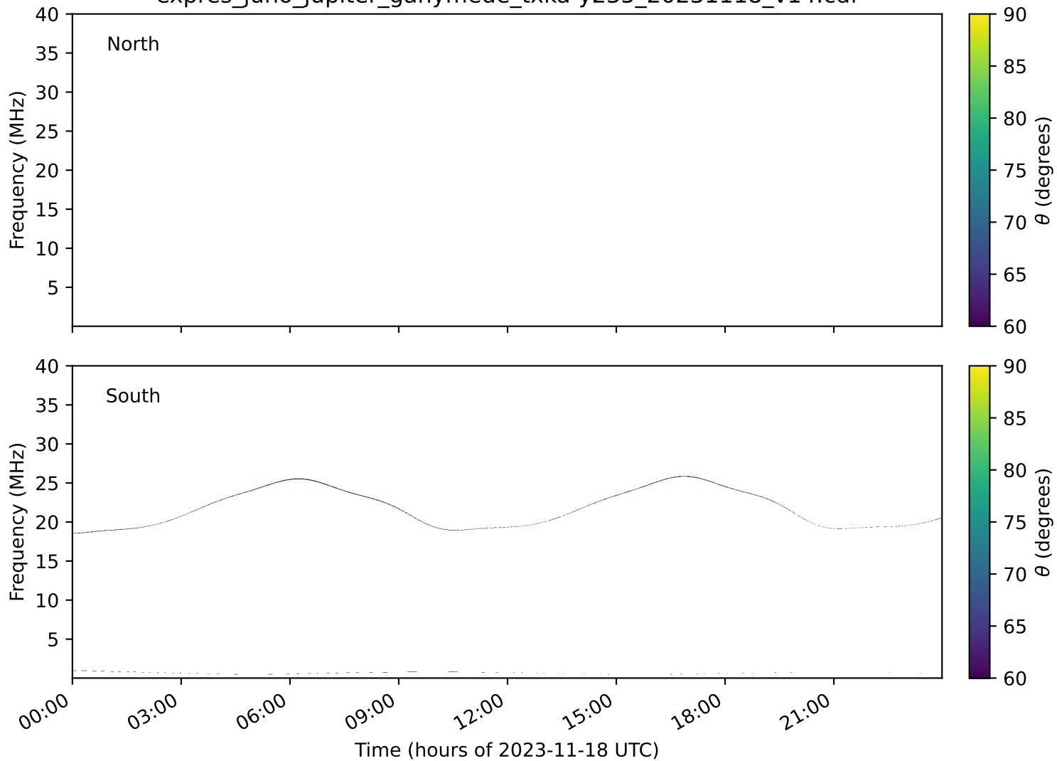
expres_juno_jupiter_ganymede_txka-y235_20231118_v14.cdf
