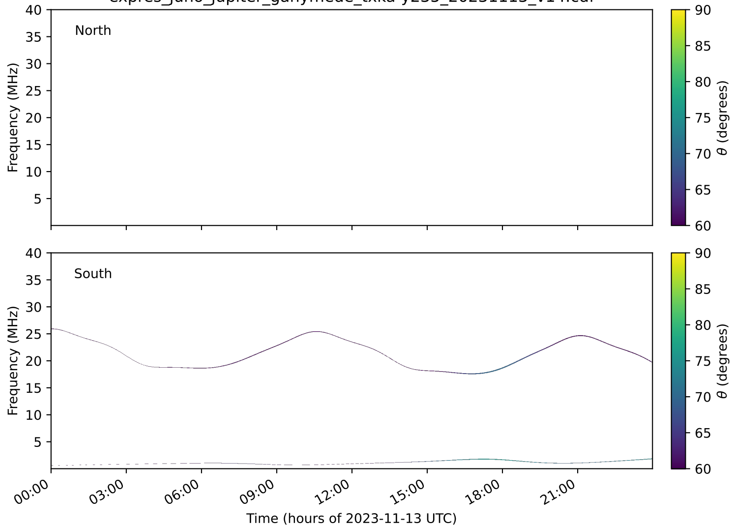
expres_juno_jupiter_ganymede_txka-y235_20231113_v14.cdf
