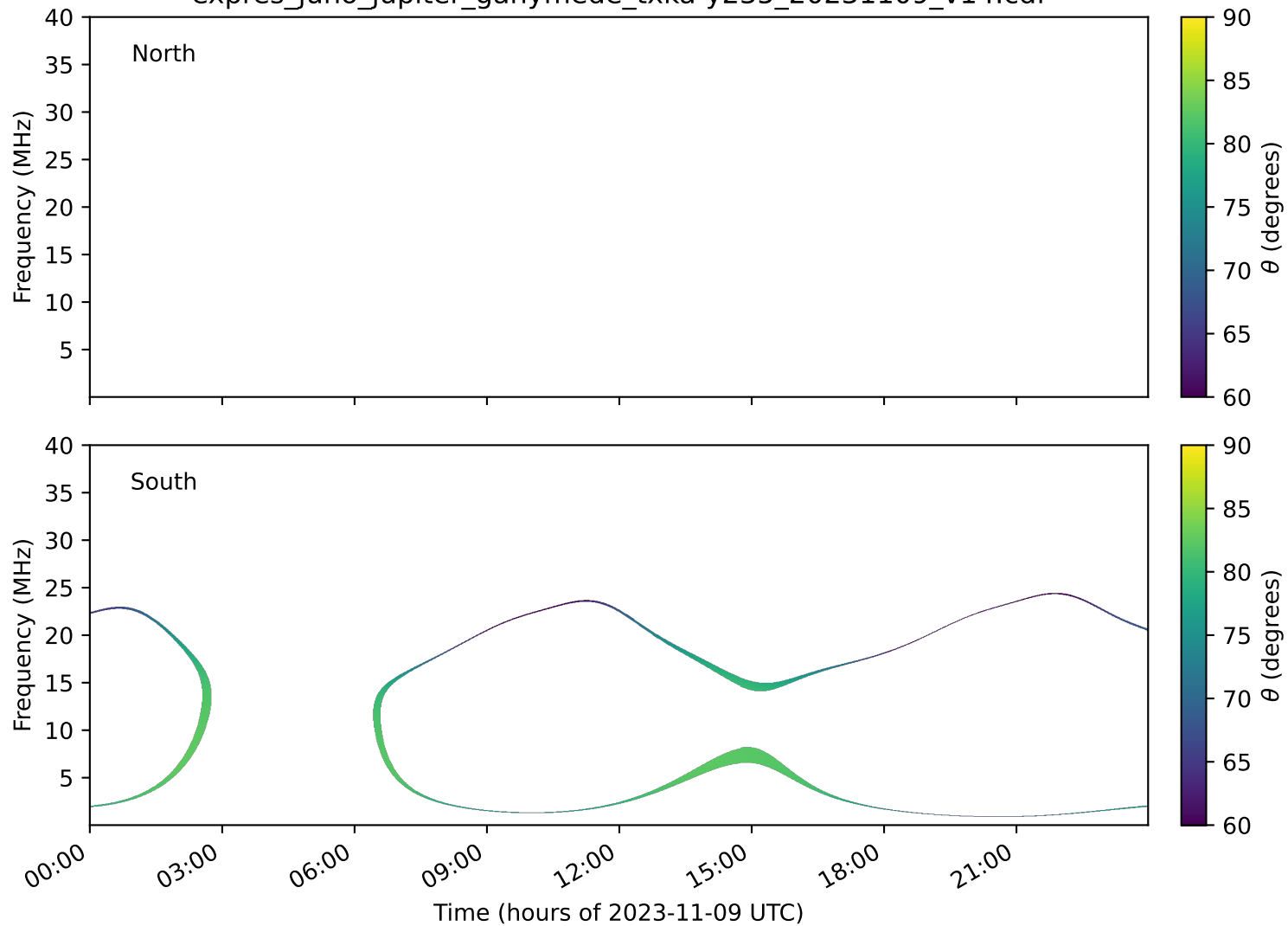
expres_juno_jupiter_ganymede_txka-y235_20231109_v14.cdf
