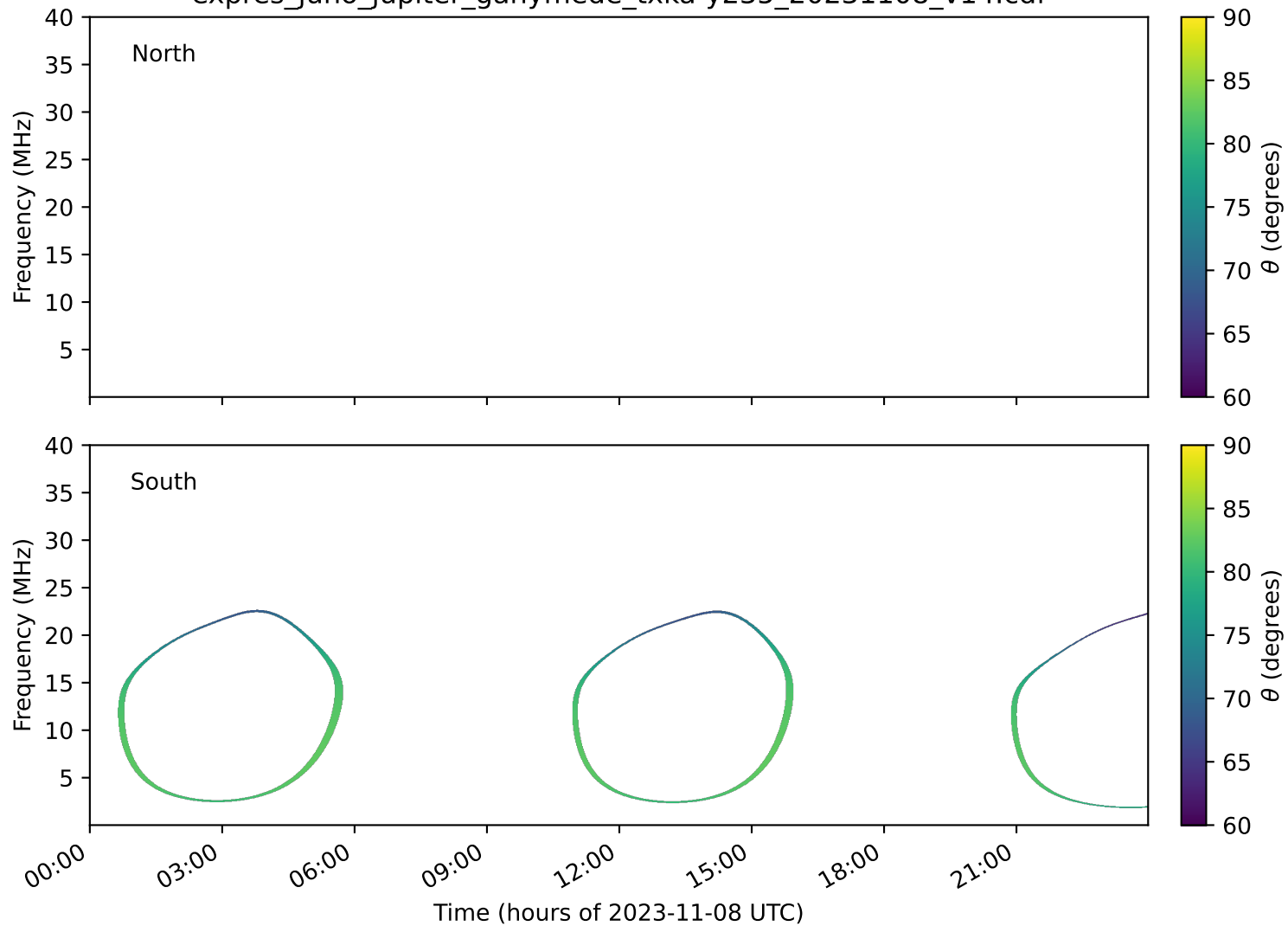
expres_juno_jupiter_ganymede_txka-y235_20231108_v14.cdf
