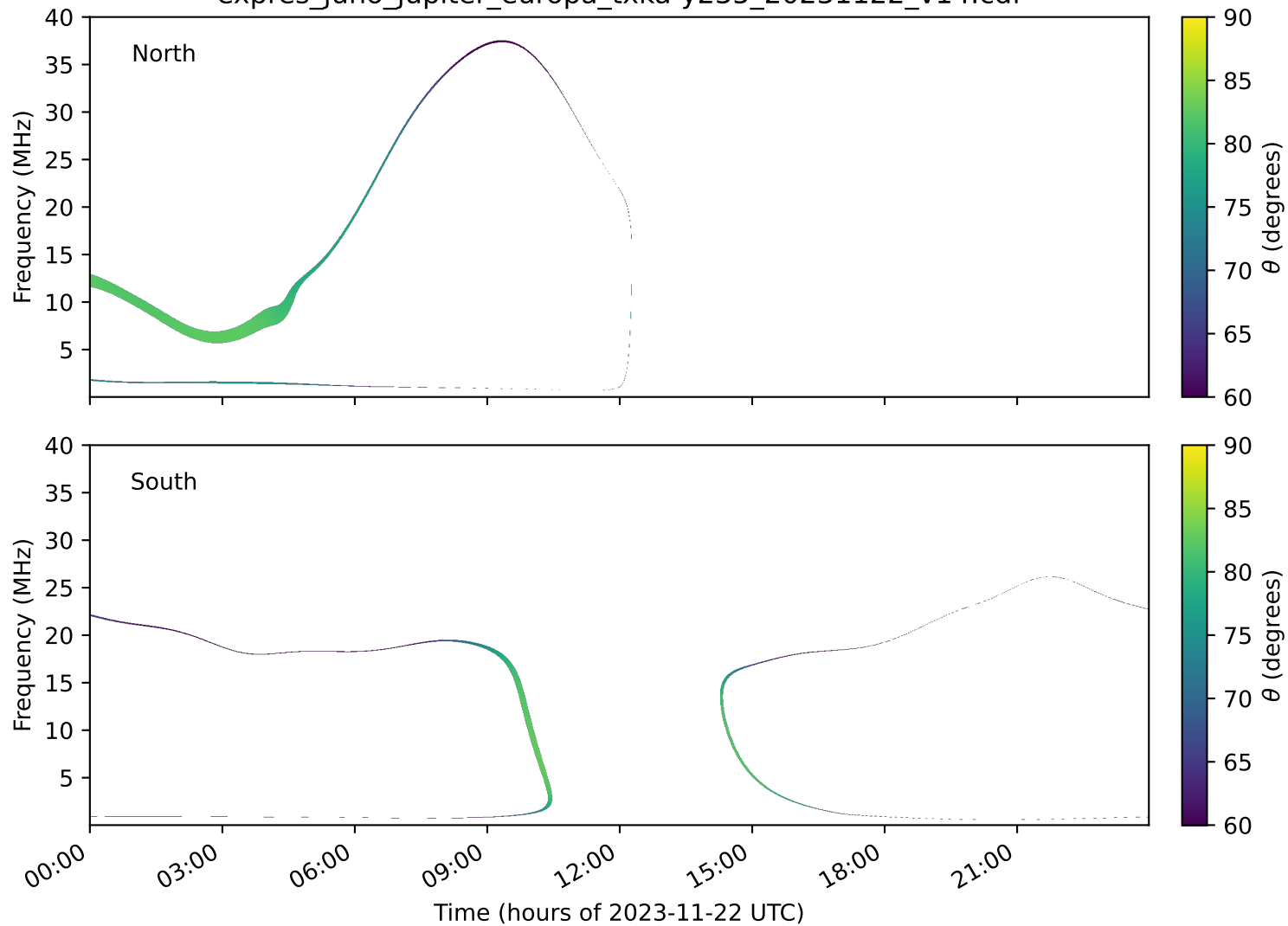
expres_juno_jupiter_europa_txka-y235_20231122_v14.cdf
