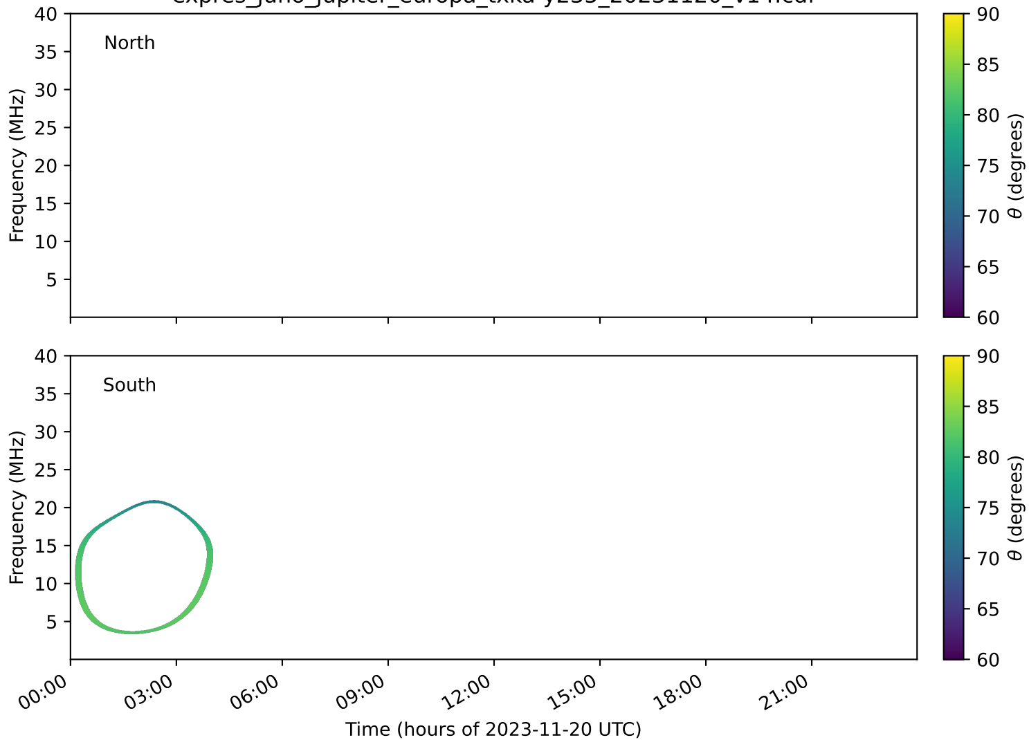
expres_juno_jupiter_europa_txka-y235_20231120_v14.cdf
