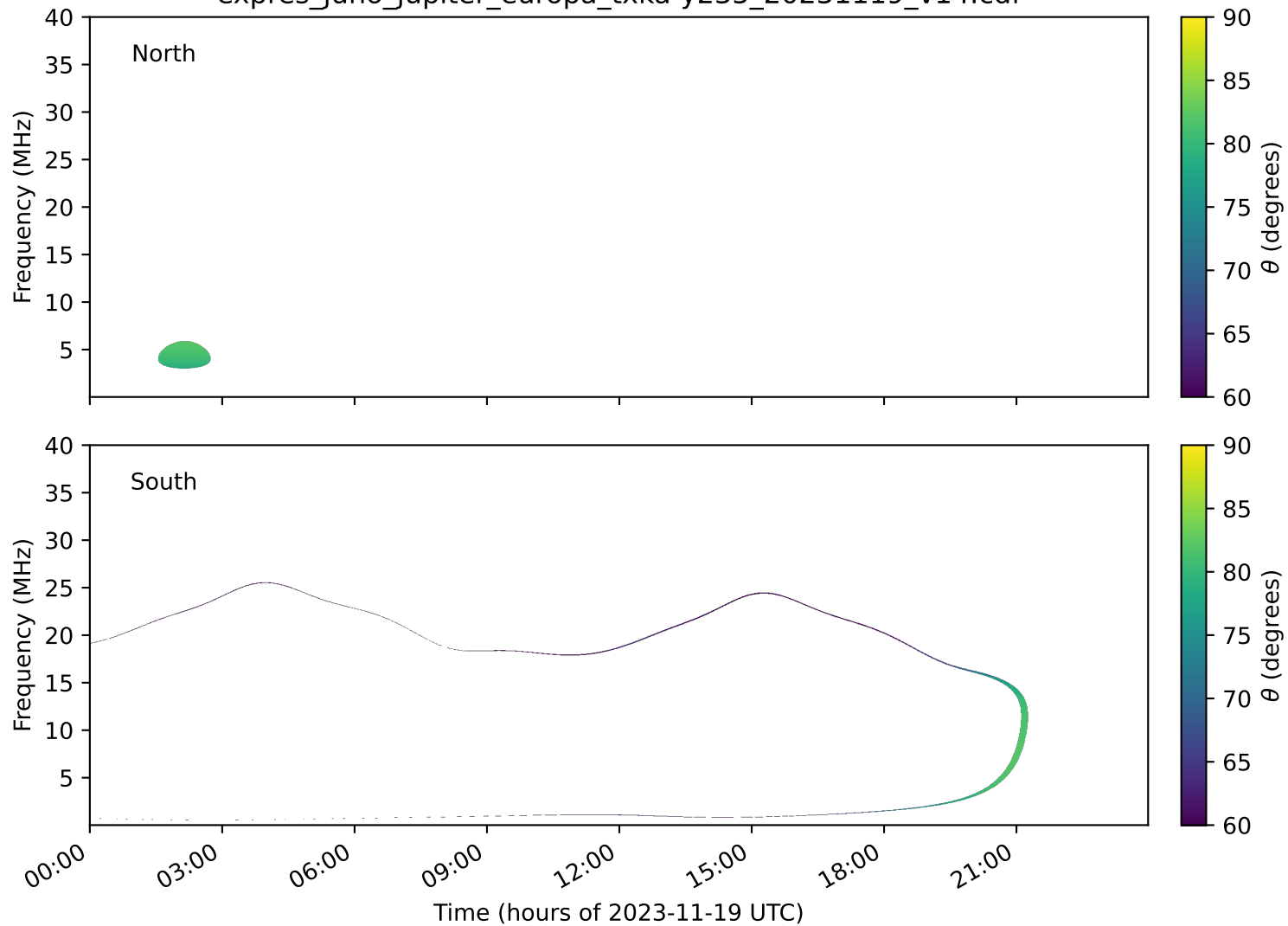
expres_juno_jupiter_europa_txka-y235_20231119_v14.cdf
