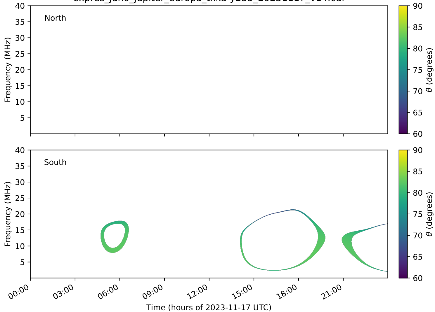
expres_juno_jupiter_europa_txka-y235_20231117_v14.cdf
