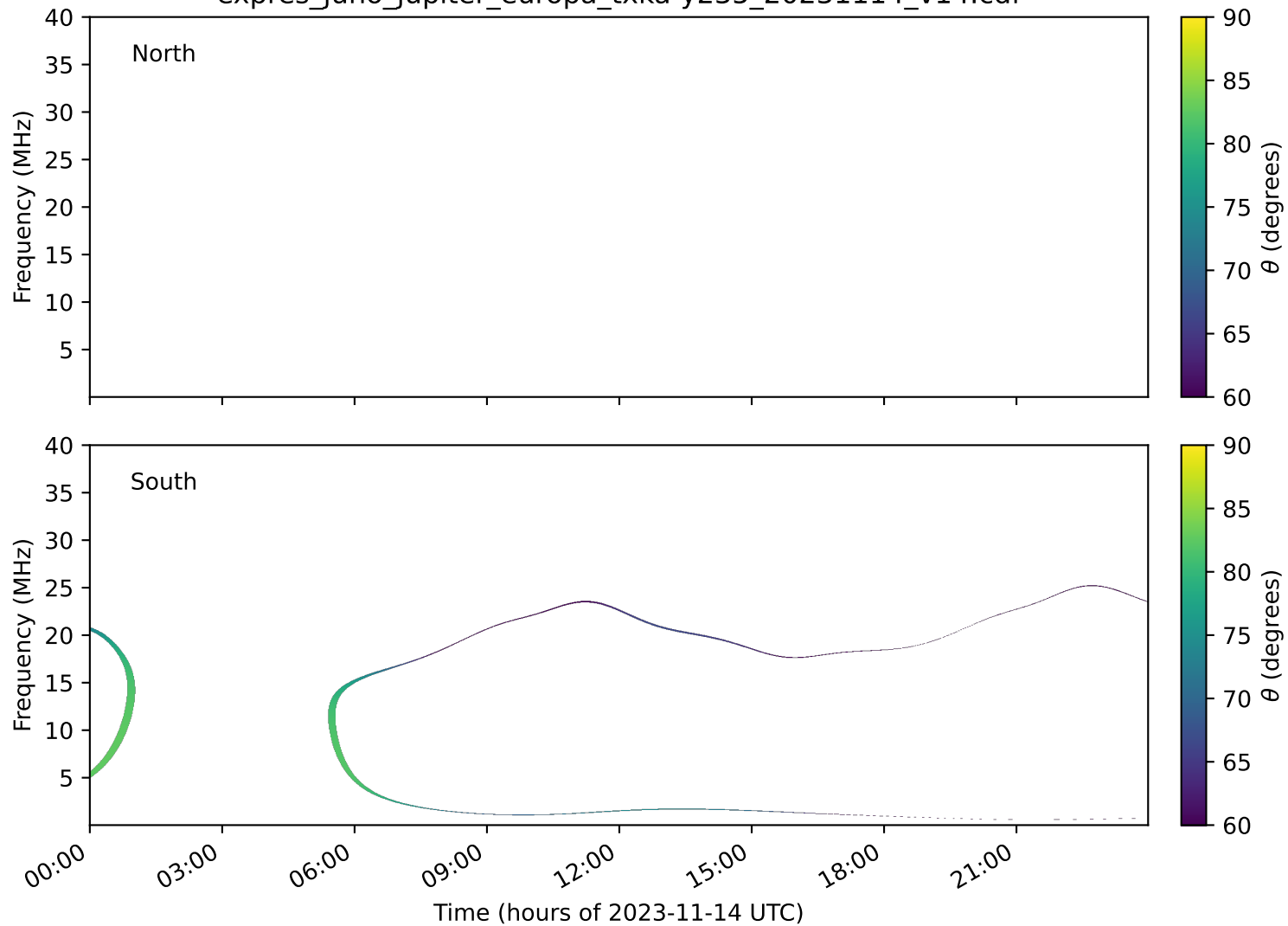
expres_juno_jupiter_europa_txka-y235_20231114_v14.cdf
