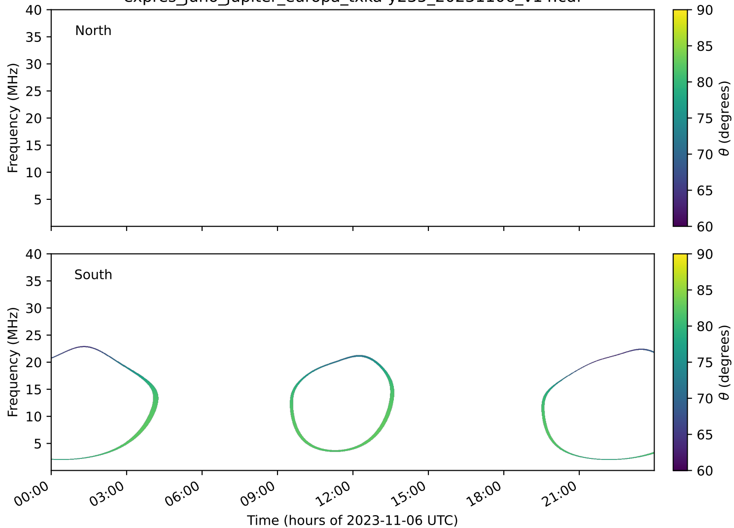
expres_juno_jupiter_europa_txka-y235_20231106_v14.cdf
