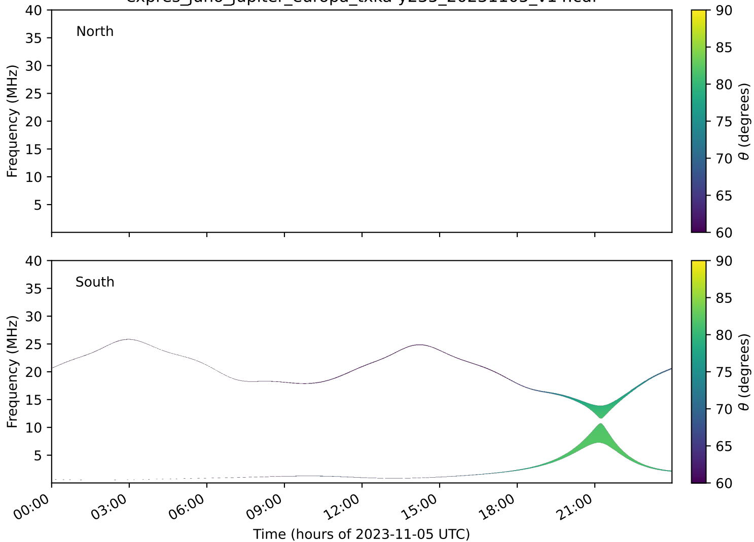
expres_juno_jupiter_europa_txka-y235_20231105_v14.cdf
