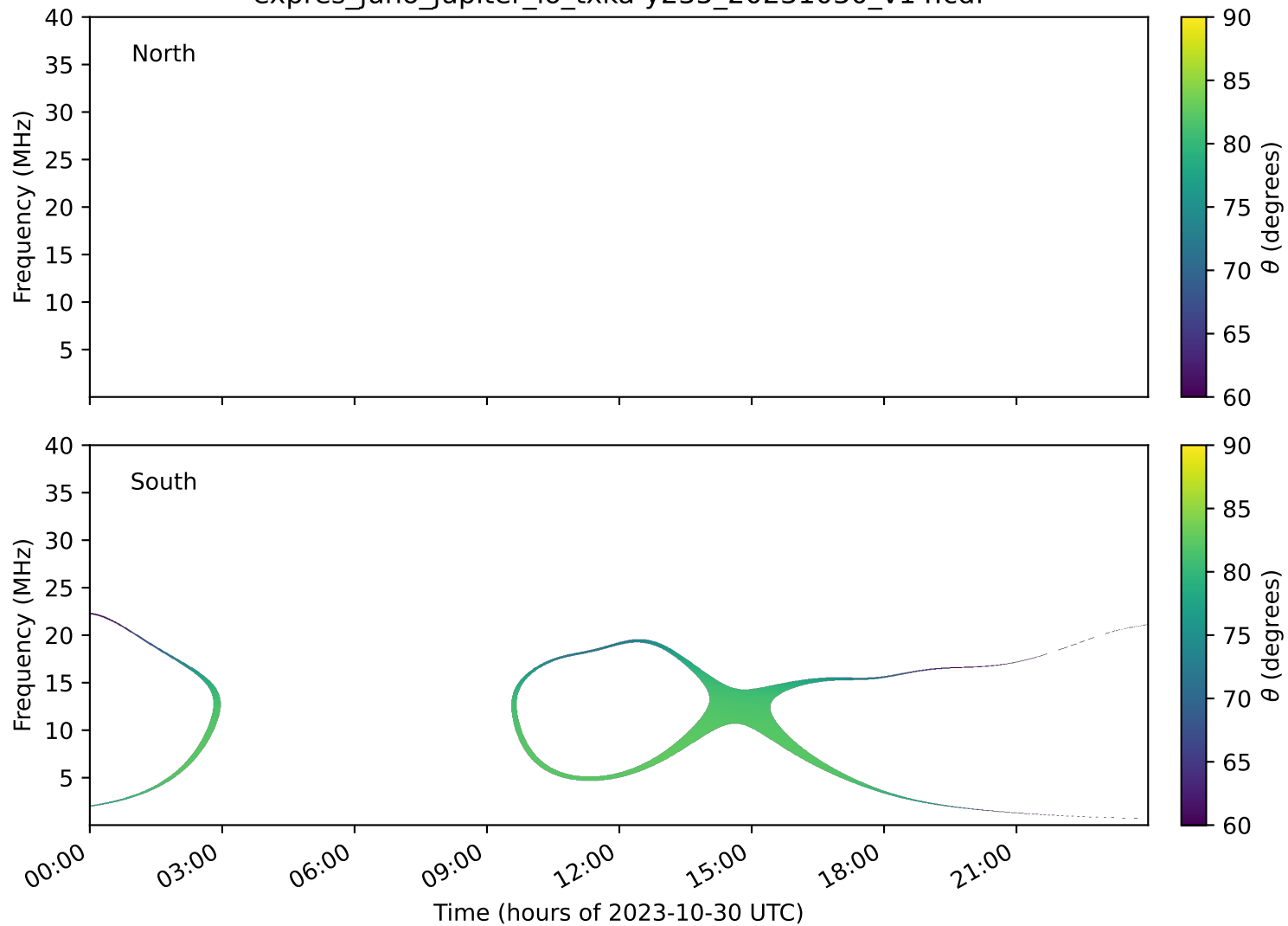
expres_juno_jupiter_io_txka-y235_20231030_v14.cdf
