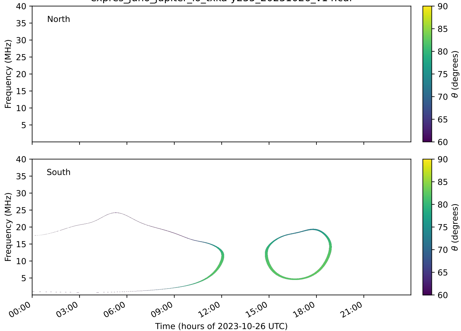
expres_juno_jupiter_io_txka-y235_20231026_v14.cdf
