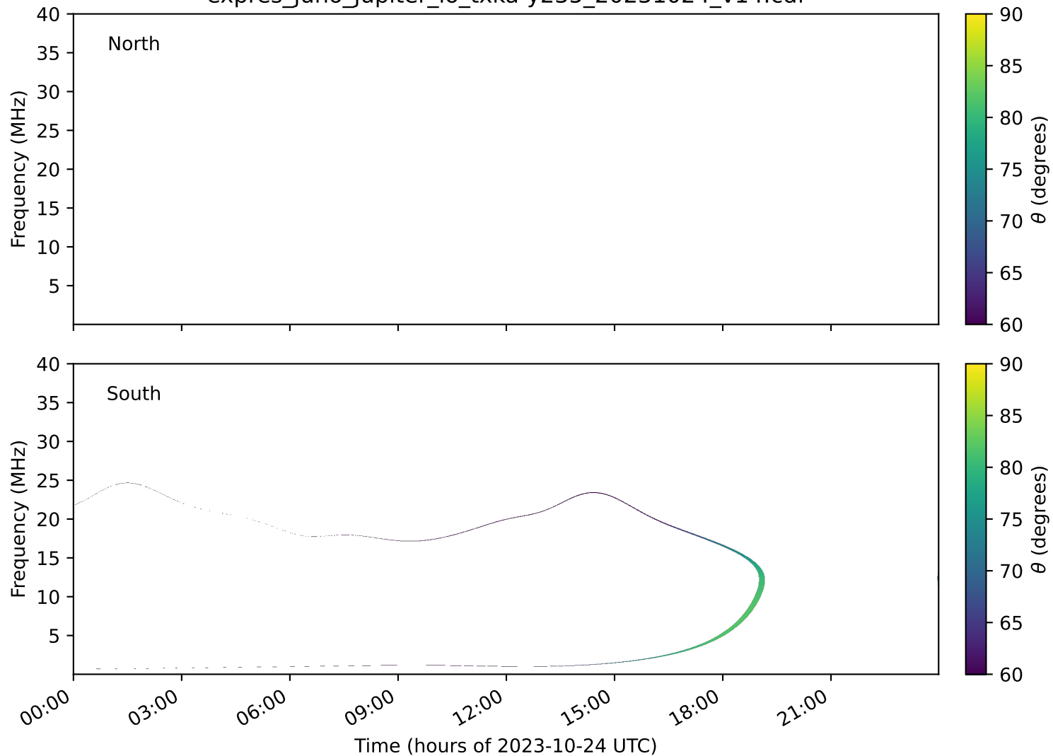
expres_juno_jupiter_io_txka-y235_20231024_v14.cdf
