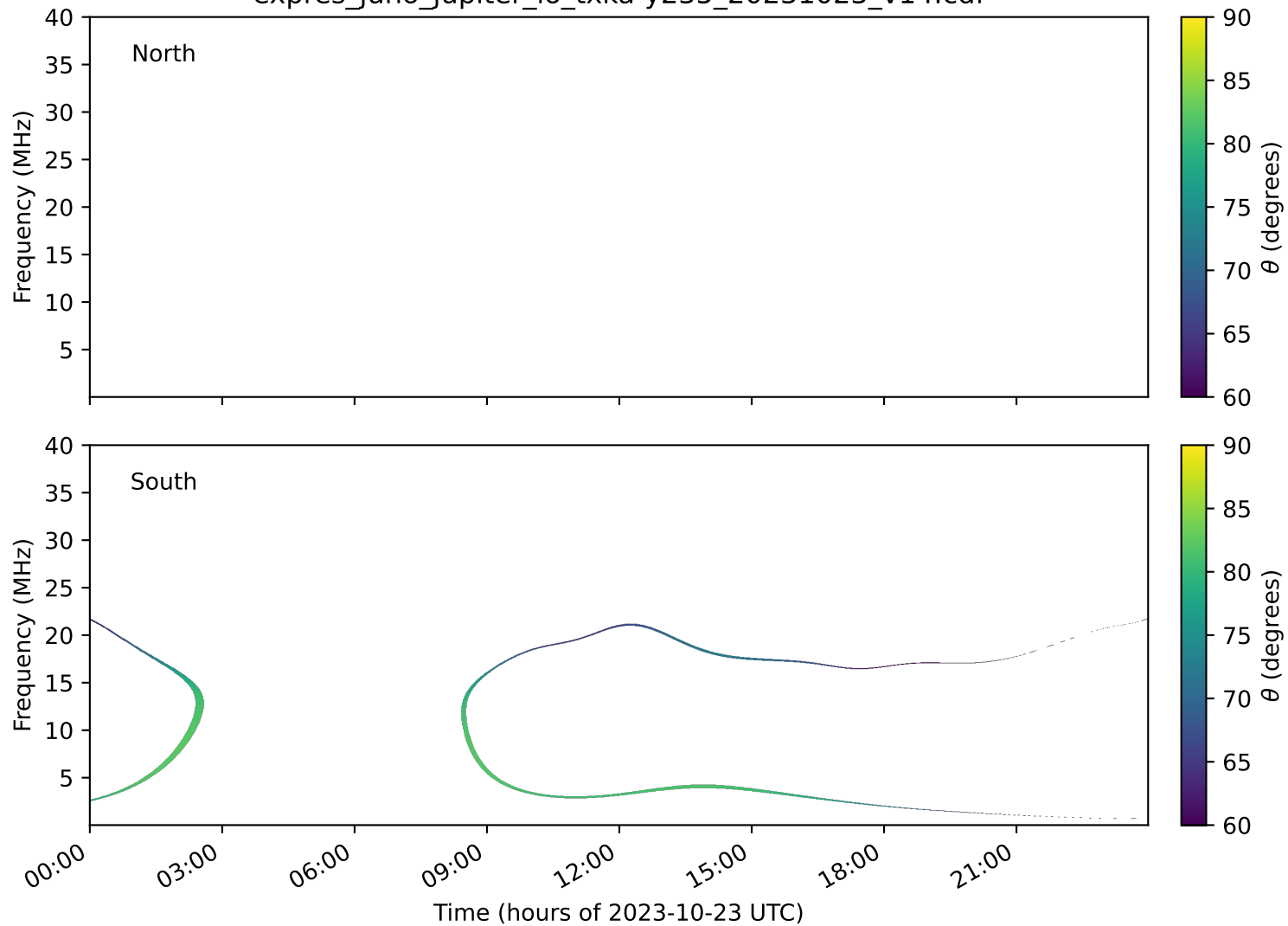
expres_juno_jupiter_io_txka-y235_20231023_v14.cdf
