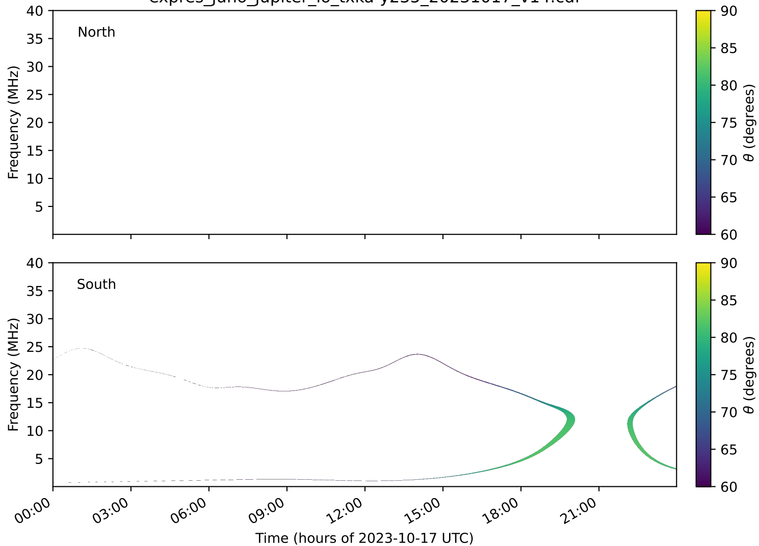
expres_juno_jupiter_io_txka-y235_20231017_v14.cdf
