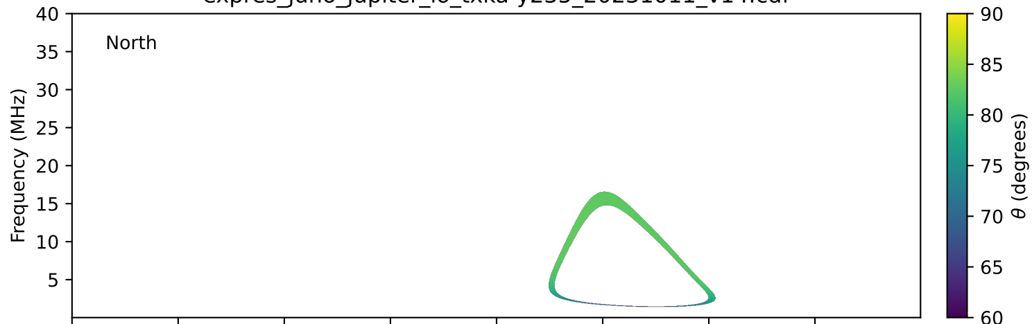
expres_juno_jupiter_io_txka-y235_20231011_v14.cdf
