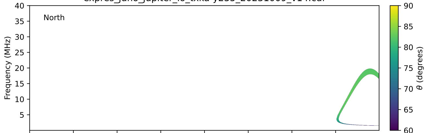
expres_juno_jupiter_io_txka-y235_20231009_v14.cdf
