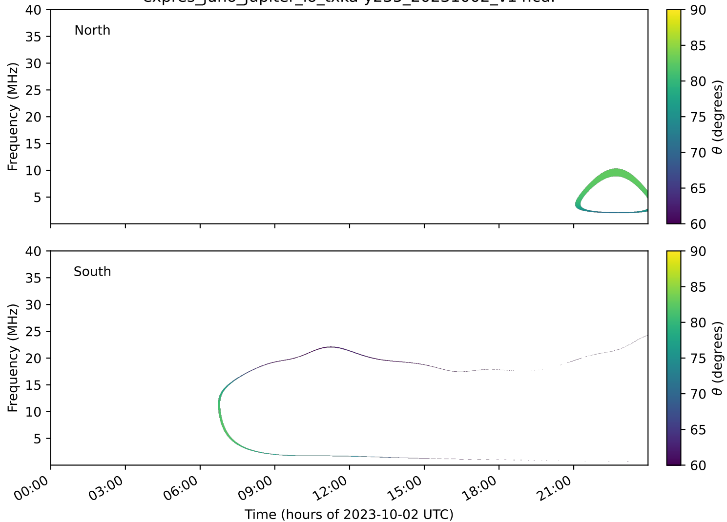
expres_juno_jupiter_io_txka-y235_20231002_v14.cdf
