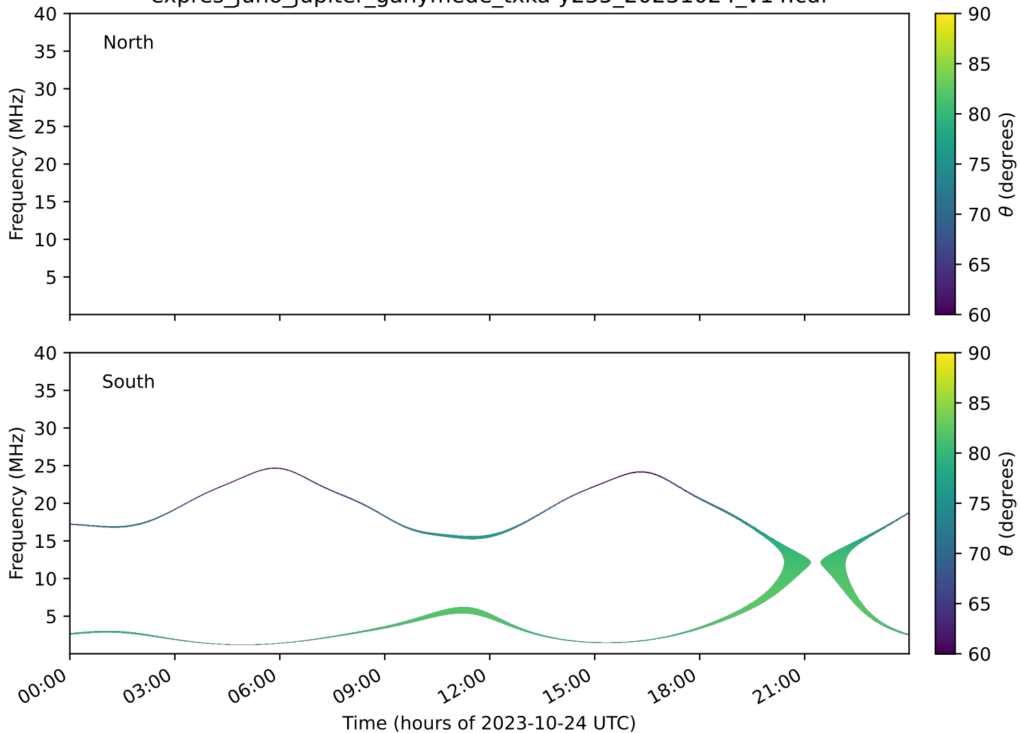
expres_juno_jupiter_ganymede_txka-y235_20231024_v14.cdf
