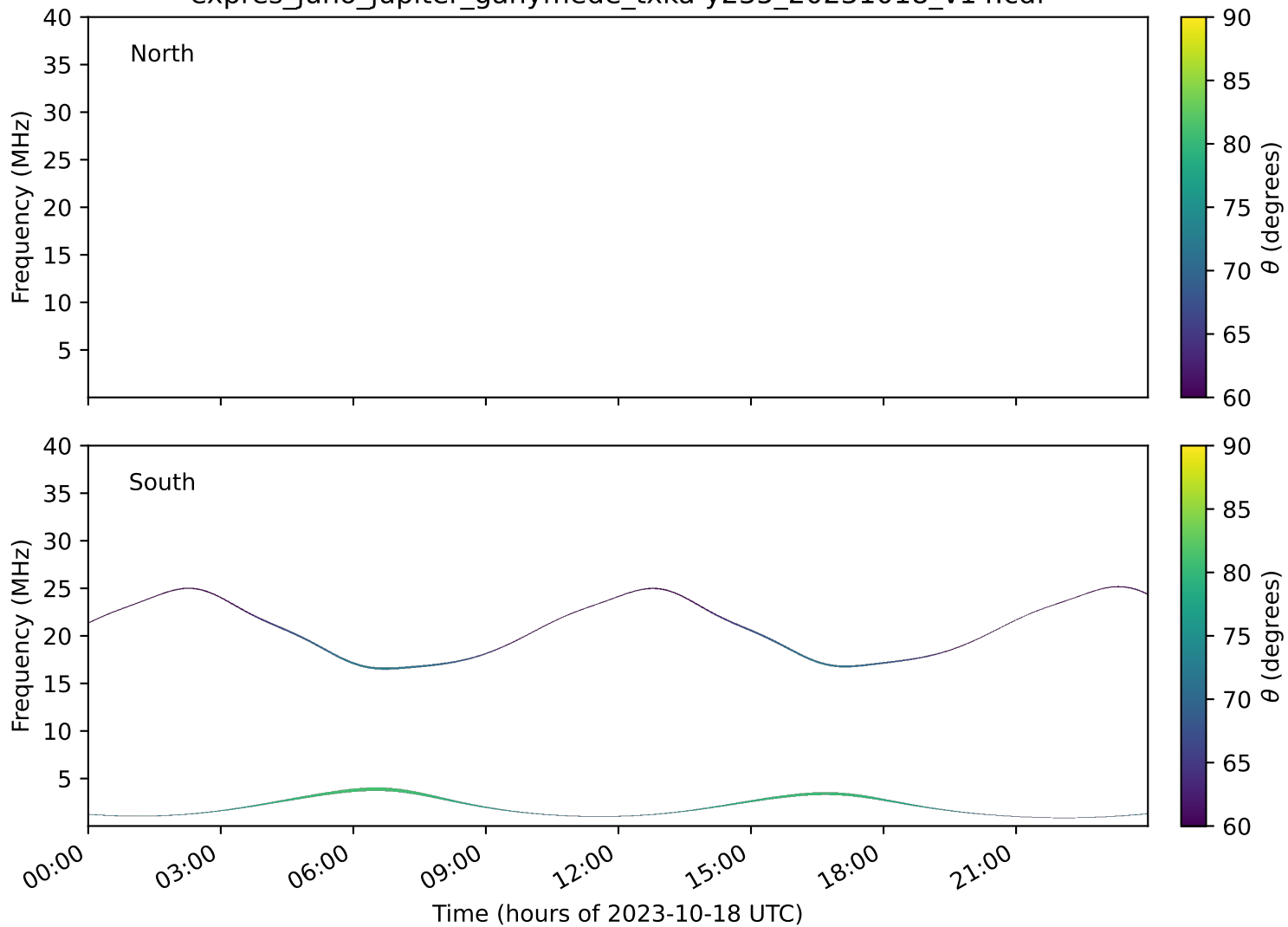
expres_juno_jupiter_ganymede_txka-y235_20231018_v14.cdf
