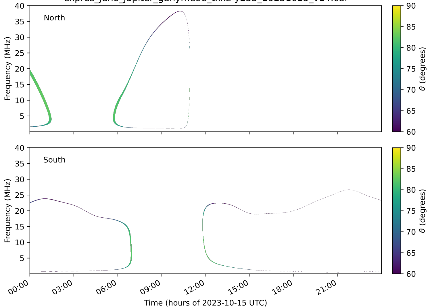
expres_juno_jupiter_ganymede_txka-y235_20231015_v14.cdf
