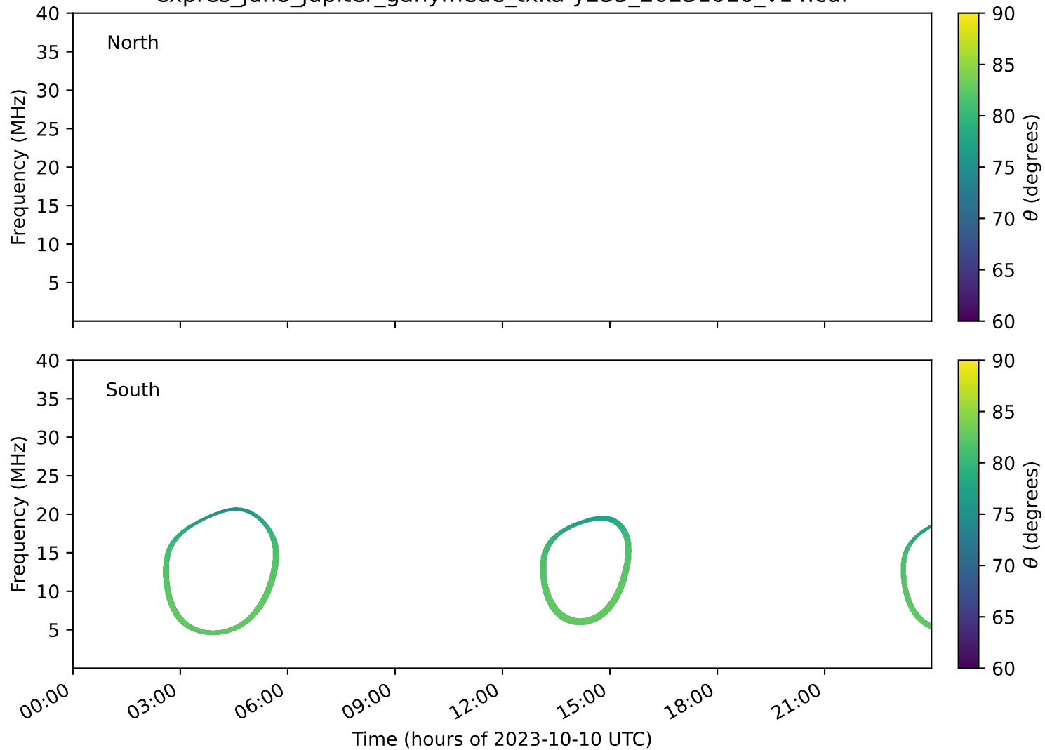
expres_juno_jupiter_ganymede_txka-y235_20231010_v14.cdf
