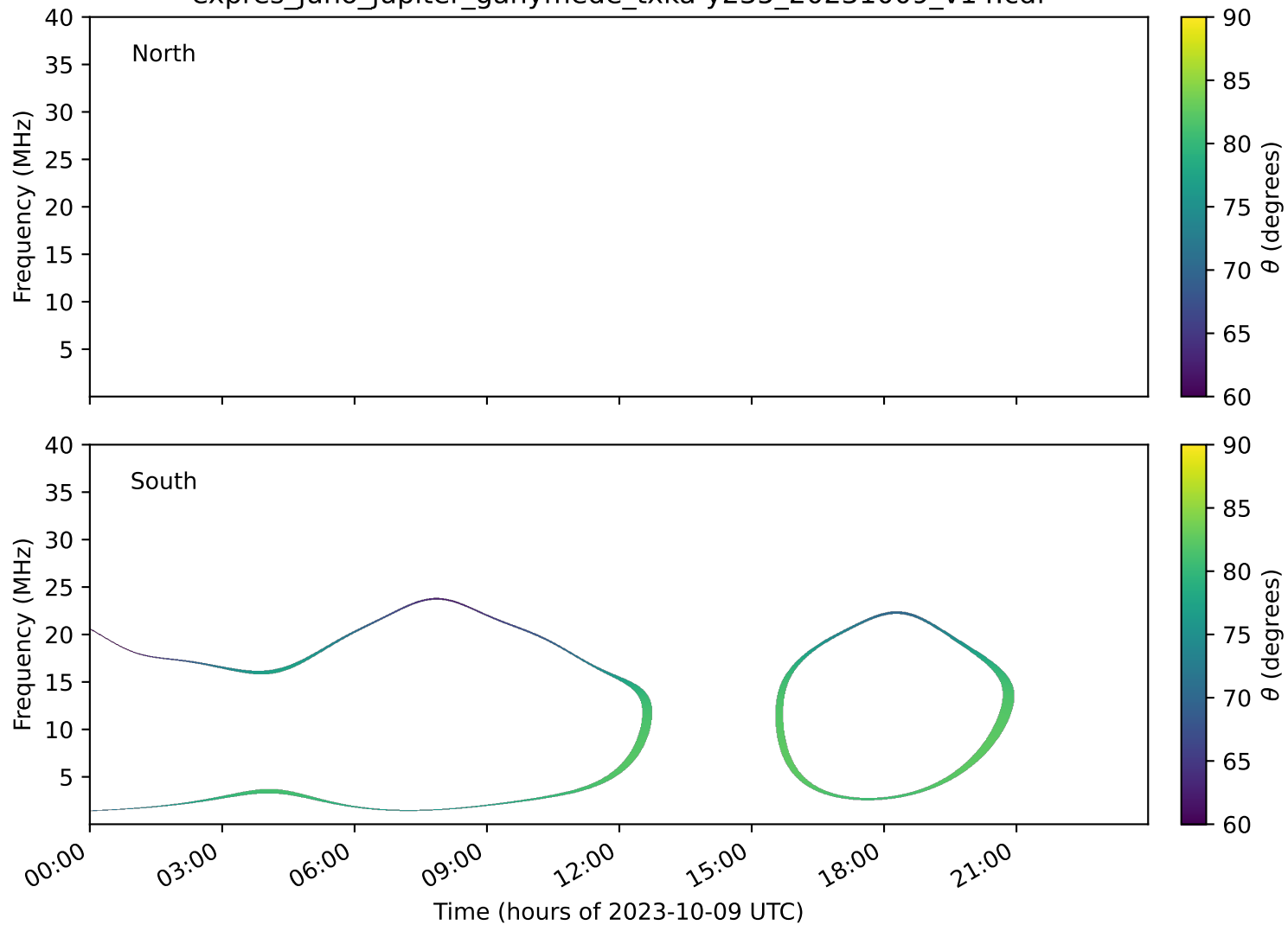
expres_juno_jupiter_ganymede_txka-y235_20231009_v14.cdf
