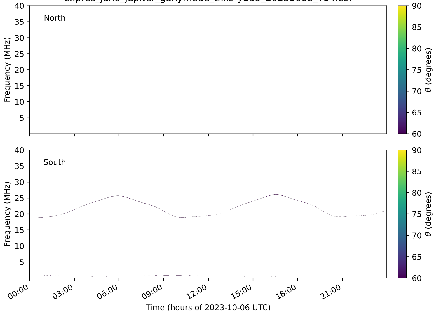
expres_juno_jupiter_ganymede_txka-y235_20231006_v14.cdf
