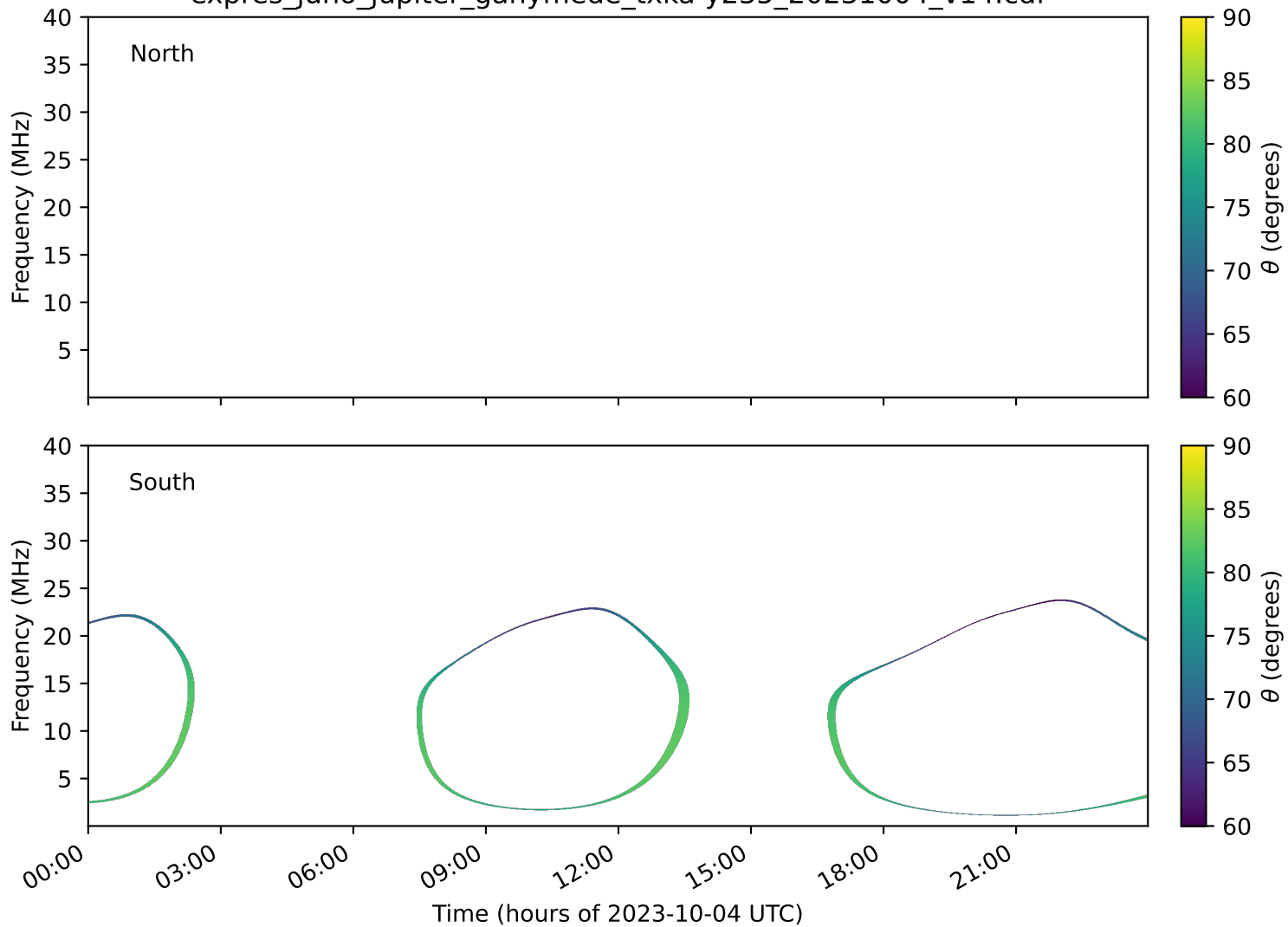
expres_juno_jupiter_ganymede_txka-y235_20231004_v14.cdf
