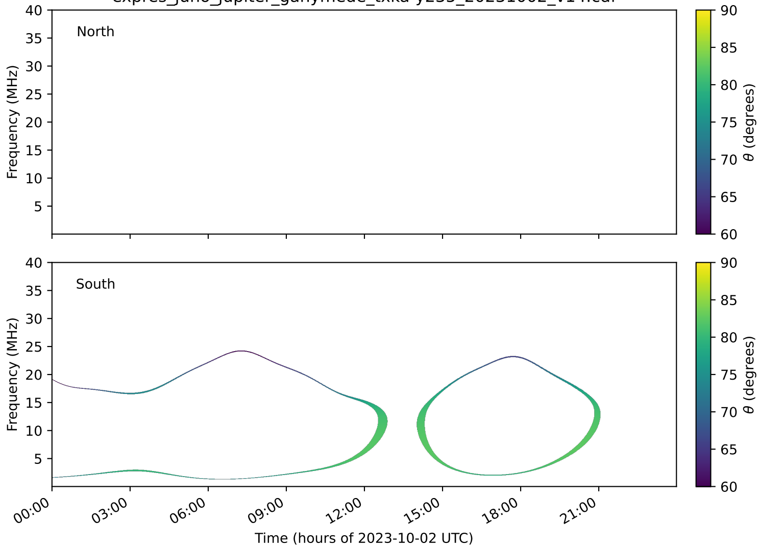
expres_juno_jupiter_ganymede_txka-y235_20231002_v14.cdf
