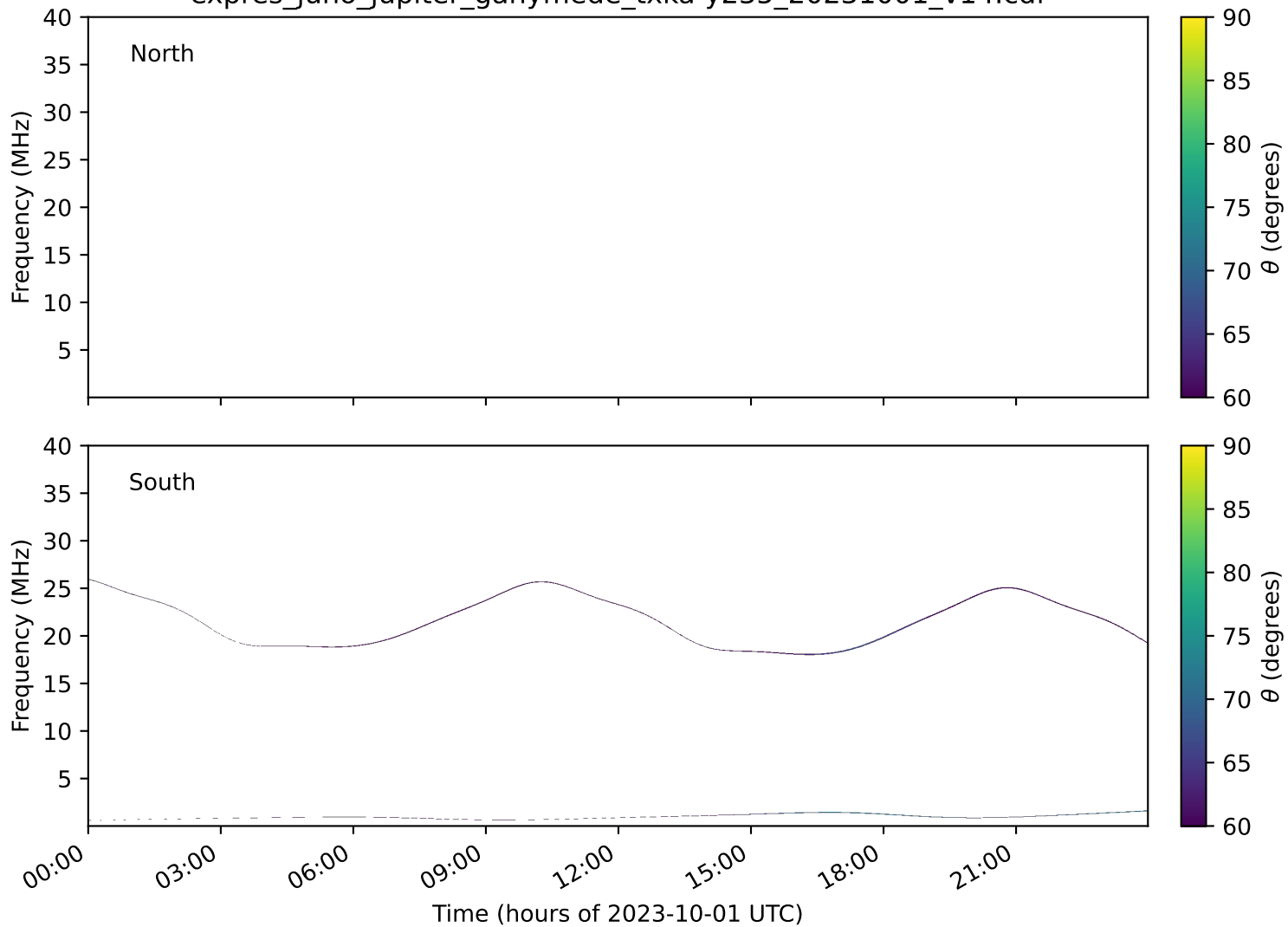
expres_juno_jupiter_ganymede_txka-y235_20231001_v14.cdf
