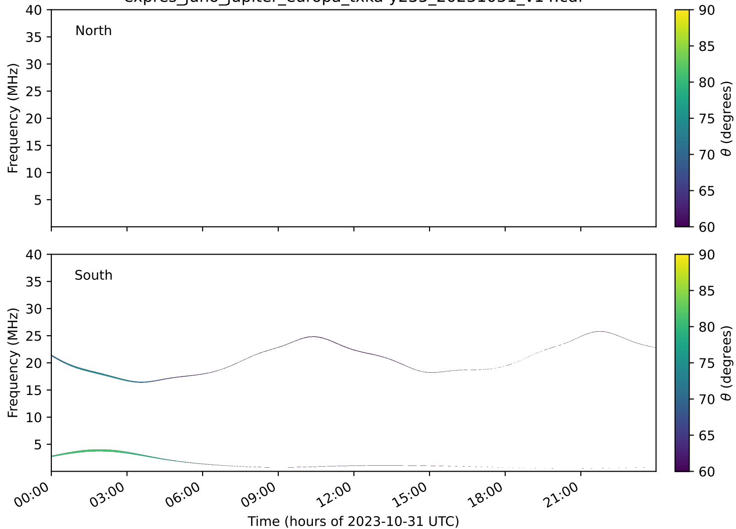
expres_juno_jupiter_europa_txka-y235_20231031_v14.cdf
