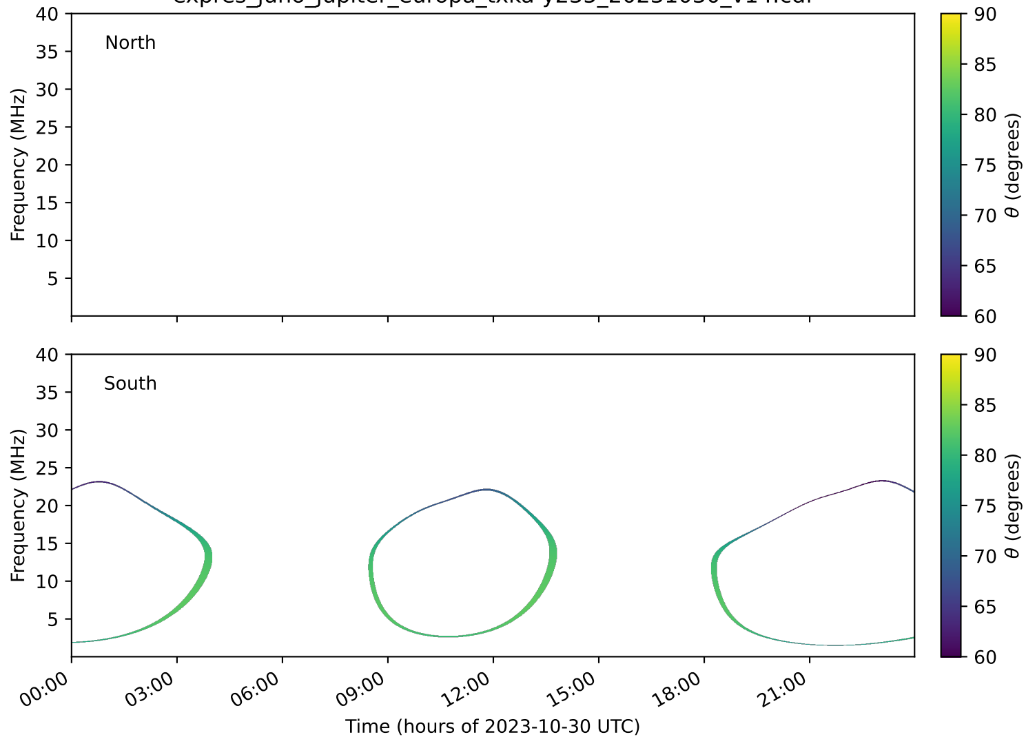
expres_juno_jupiter_europa_txka-y235_20231030_v14.cdf
