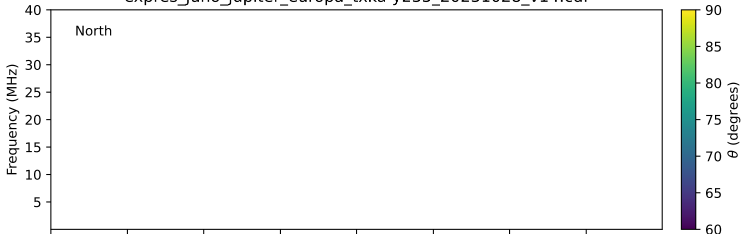
expres_juno_jupiter_europa_txka-y235_20231028_v14.cdf
