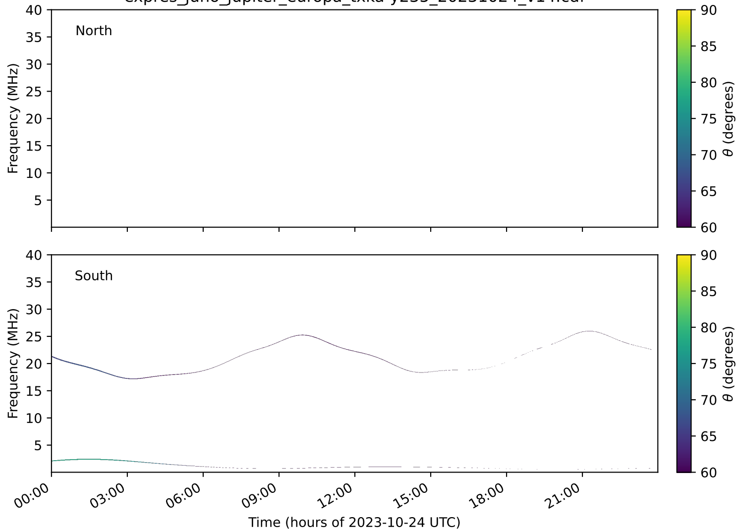
expres_juno_jupiter_europa_txka-y235_20231024_v14.cdf
