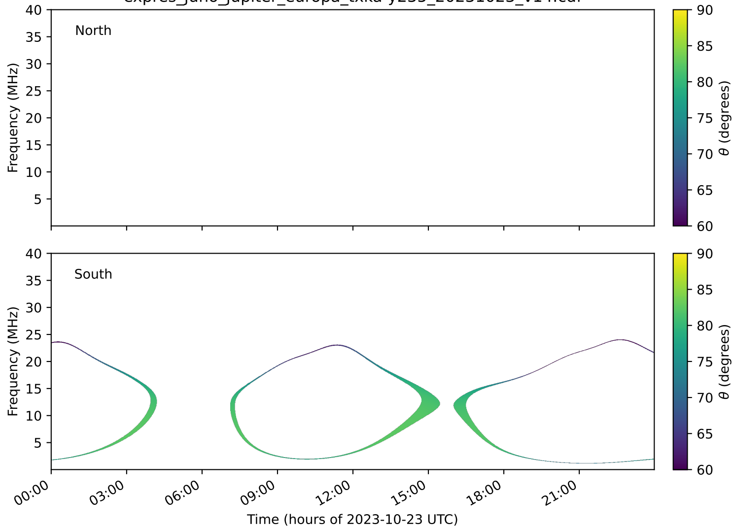
expres_juno_jupiter_europa_txka-y235_20231023_v14.cdf
