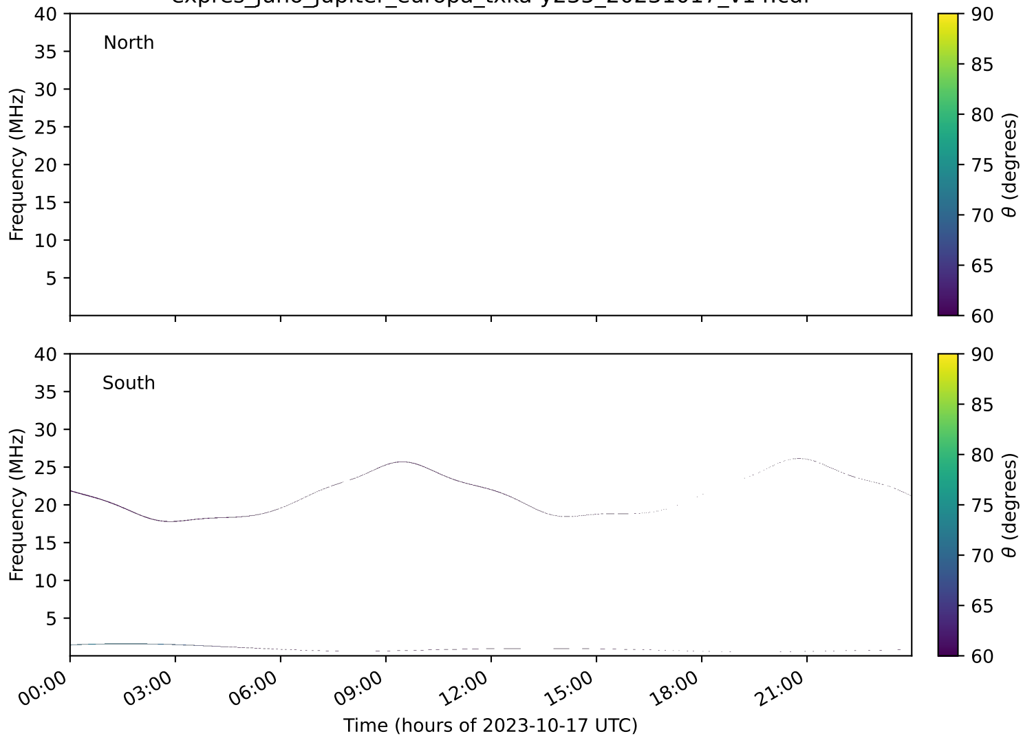
expres_juno_jupiter_europa_txka-y235_20231017_v14.cdf
