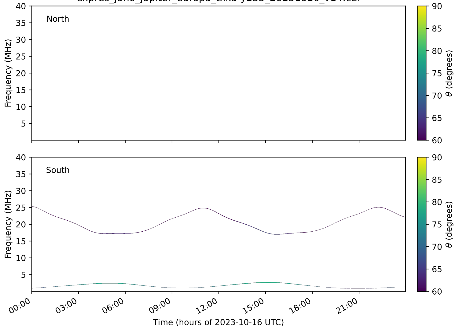
expres_juno_jupiter_europa_txka-y235_20231016_v14.cdf
