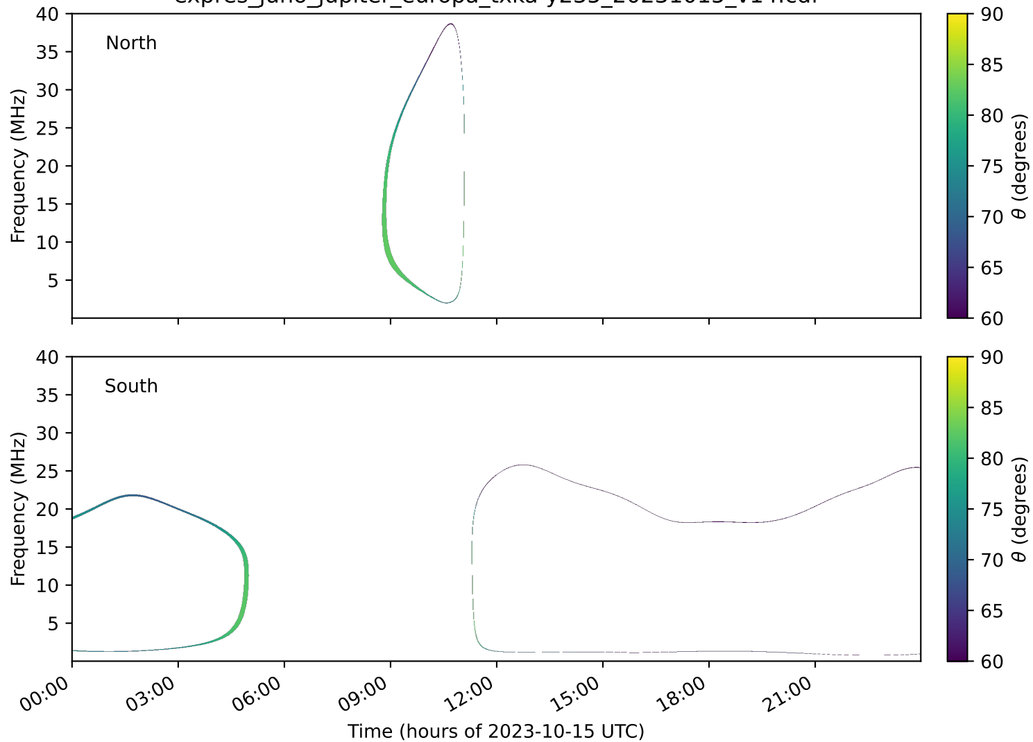
expres_juno_jupiter_europa_txka-y235_20231015_v14.cdf
