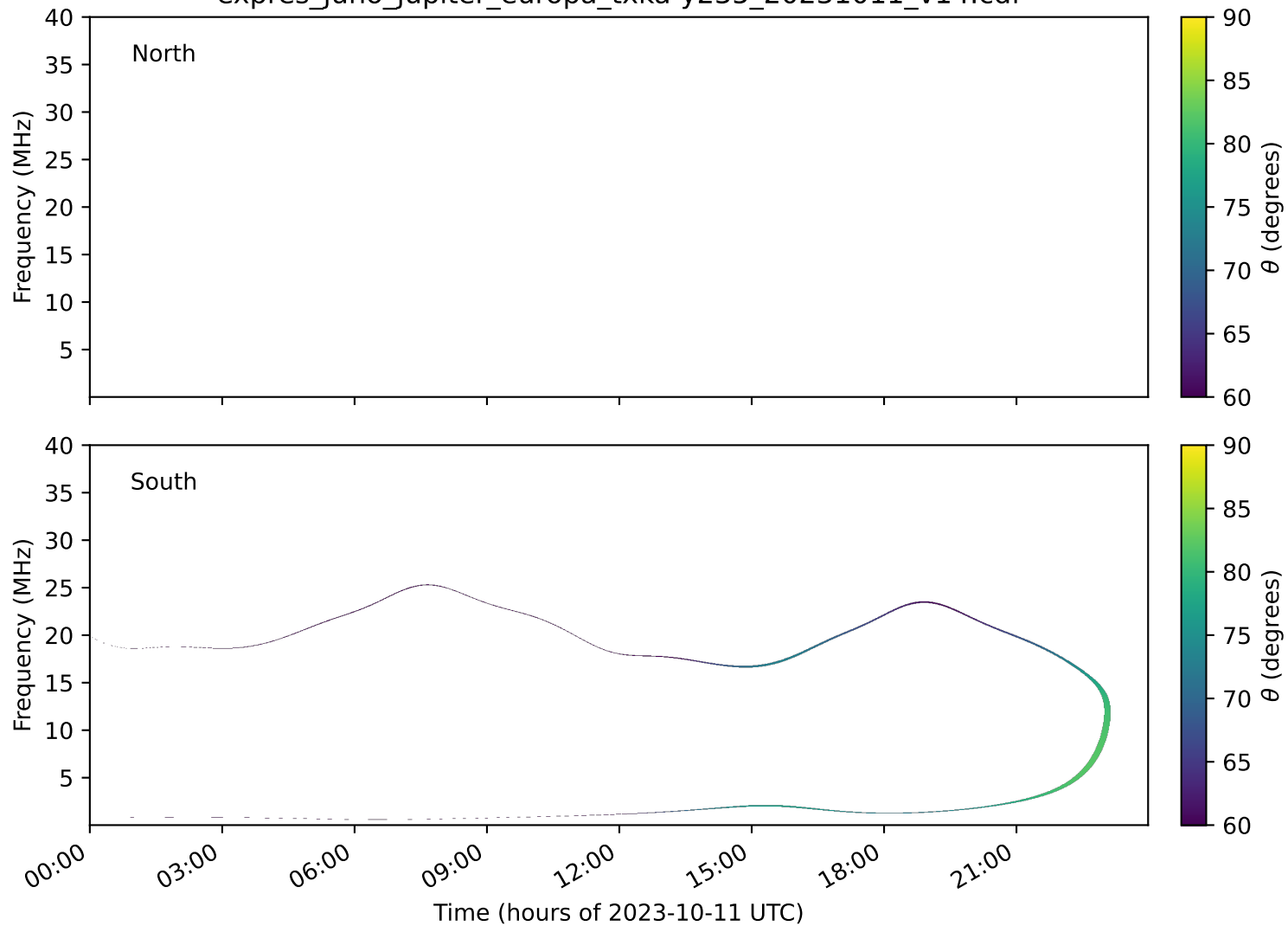
expres_juno_jupiter_europa_txka-y235_20231011_v14.cdf
