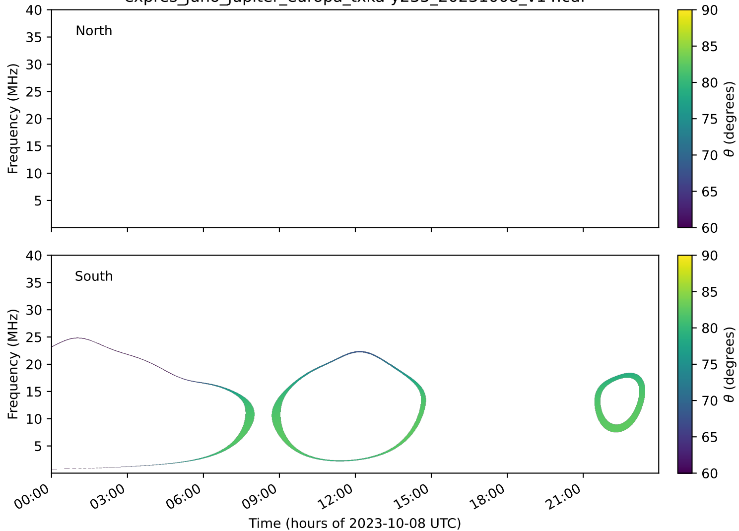
expres_juno_jupiter_europa_txka-y235_20231008_v14.cdf
