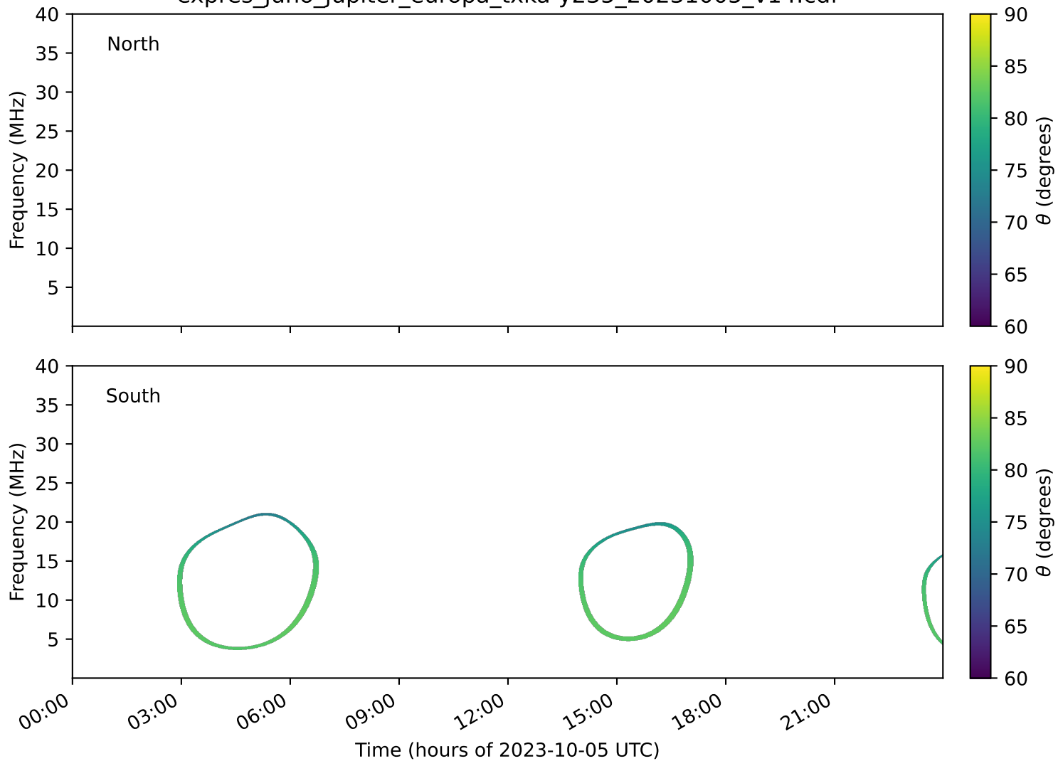
expres_juno_jupiter_europa_txka-y235_20231005_v14.cdf
