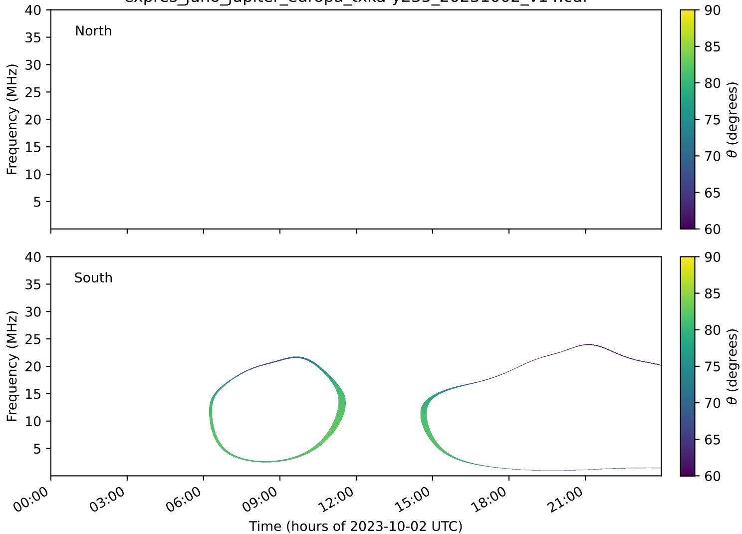
expres_juno_jupiter_europa_txka-y235_20231002_v14.cdf
