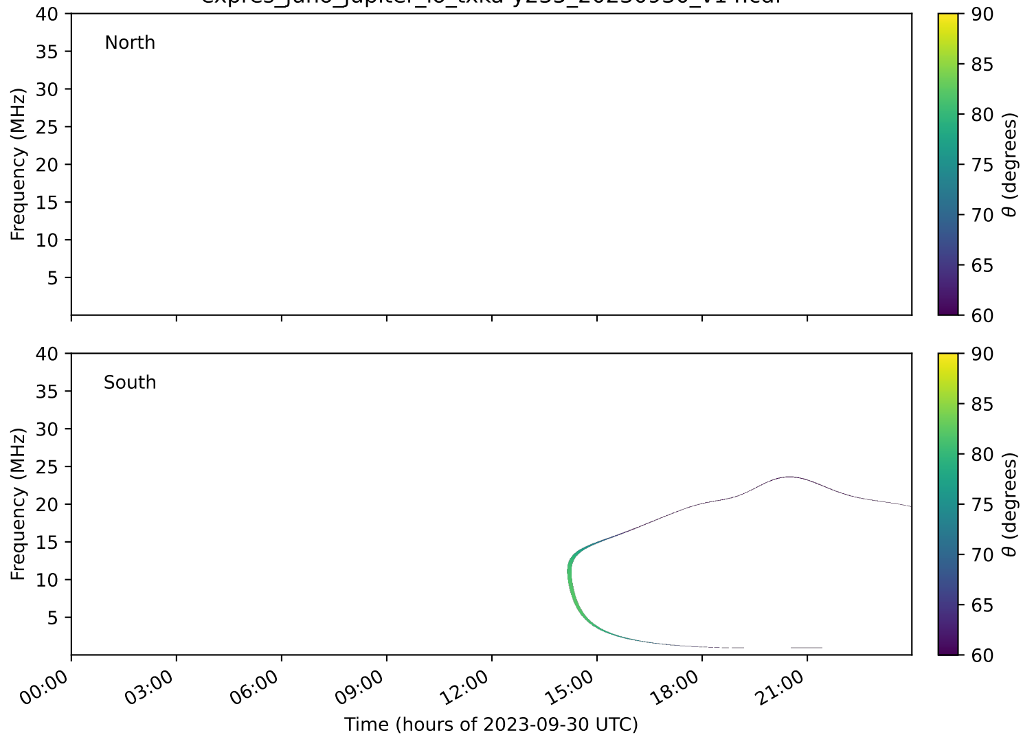
expres_juno_jupiter_io_txka-y235_20230930_v14.cdf
